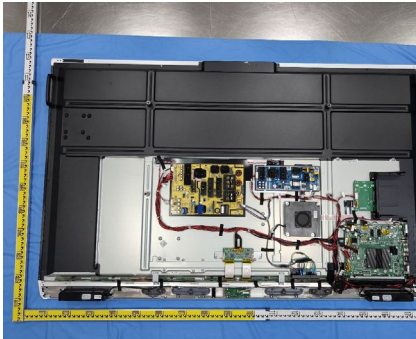
back panel removed
