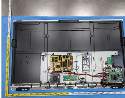
back panel removed
