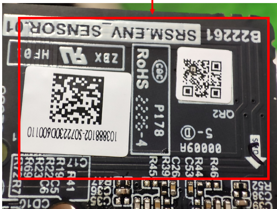
NFC Antenna 25.5mm*16.8mm
