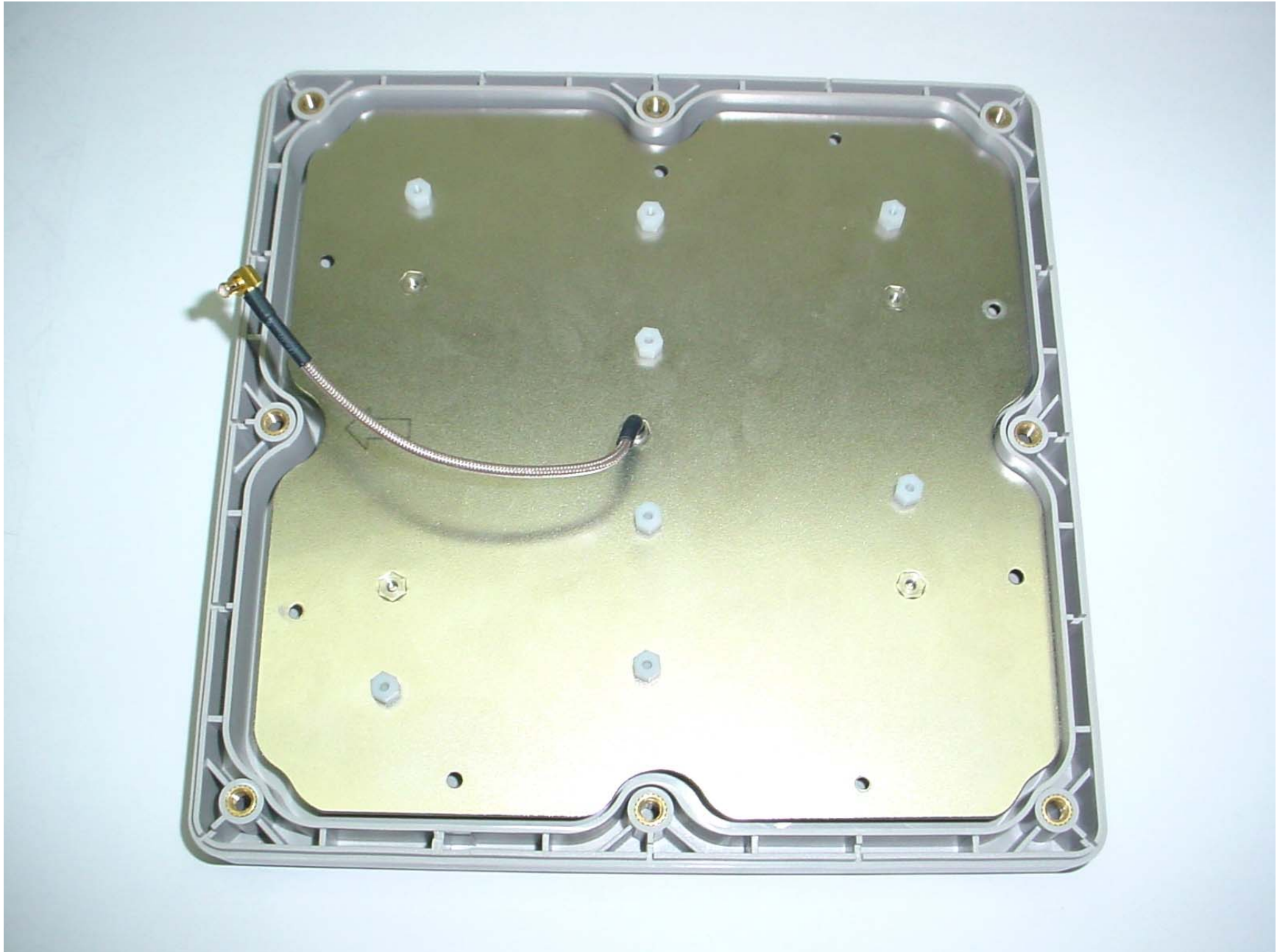
Integral Antenna
