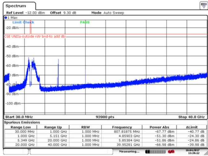
Figure 8.4-22: Spurious emissions outside restricted bands, 20 MHz channel, high channel, 10 dBi antenna, ch1, 256-QAM
