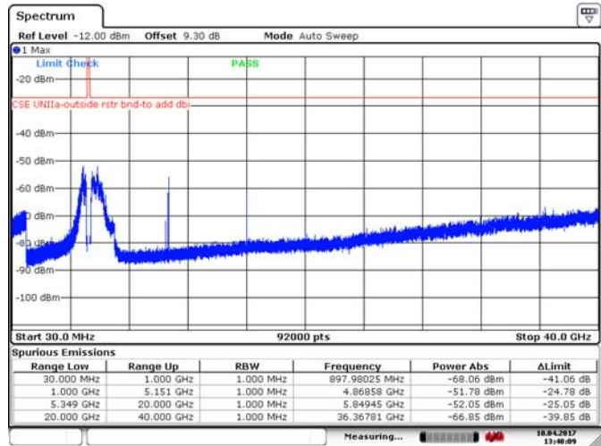
Figure 8.4-12: Spurious emissions outside restricted bands, 10 MHz channel, high channel, 10 dBi antenna, ch1, BPSK
