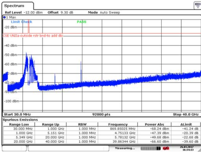
Figure 8.4-13: Spurious emissions outside restricted bands, 20 MHz channel, low channel, 10 dBi antenna, cho, 256-QAM
