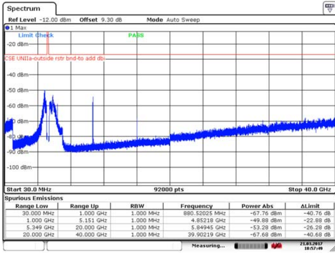
Figure 8.4-9: Spurious emissions outside restricted bands, 10 MHz channel, high channel, 10 dBi antenna, cho, 256-QAM
