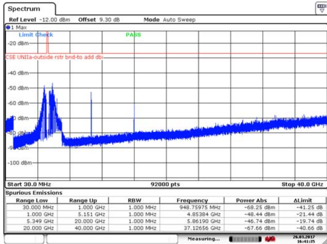
Figure 8.4-23: Spurious emissions outside restricted bands, 20 MHz channel, high channel, 10 dBi antenna, cho, BPSK
