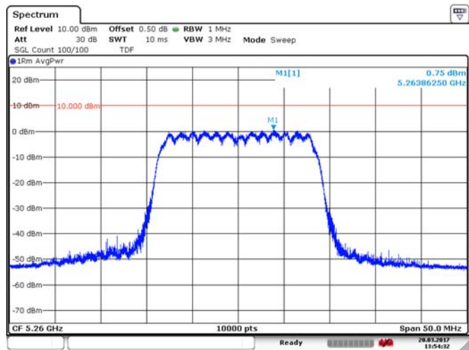
Figure 8.3-2: Sample plot for PSD on 20 MHz channel
