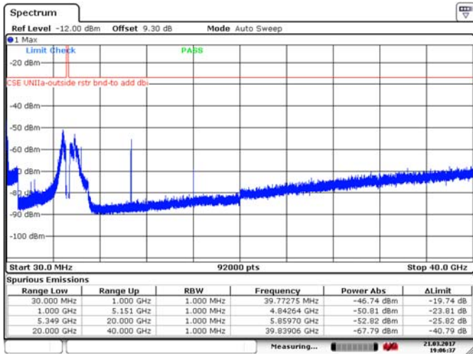
Figure 8.4-11: Spurious emissions outside restricted bands, 10 MHz channel, high channel, 10 dBi antenna, cho, BPSK
