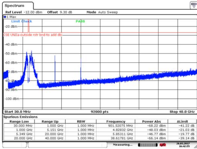
Figure 8.4-21: Spurious emissions outside restricted bands, 20 MHz channel, high channel, 10 dBi antenna, cho, 256-QAM
