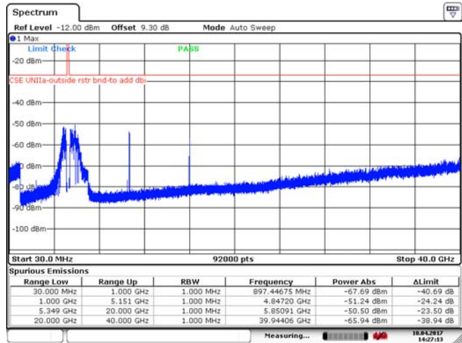
Figure 8.4-24: Spurious emissions outside restricted bands, 20 MHz channel, high channel, 10 dBi antenna, ch1, BPSK
