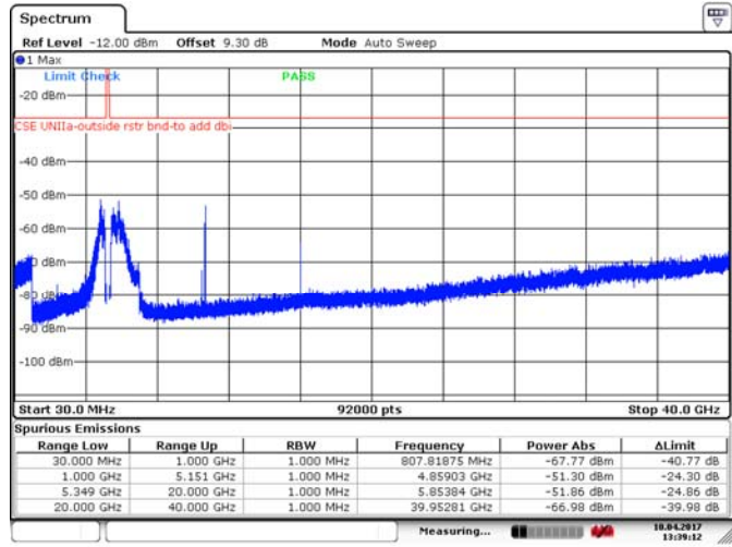
Figure 8.4-10: Spurious emissions outside restricted bands, 10 MHz channel, high channel, 10 dBi antenna, ch1, 256-QAM
