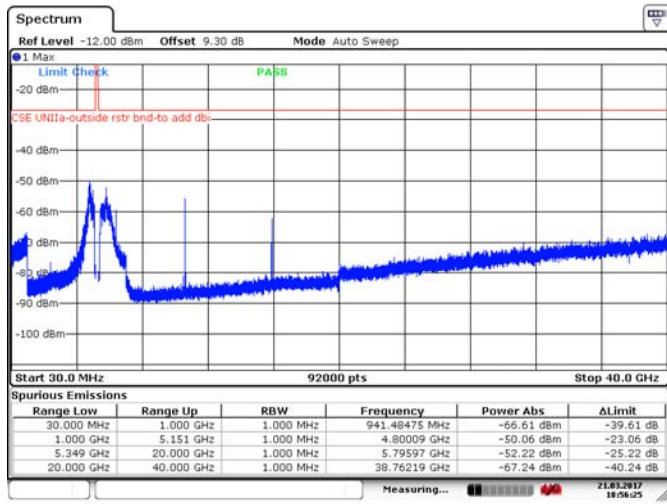
Figure 8.4-5: Spurious emissions outside restricted bands, 10 MHz channel, mid channel, 10 dBi antenna, cho, 256-QAM
