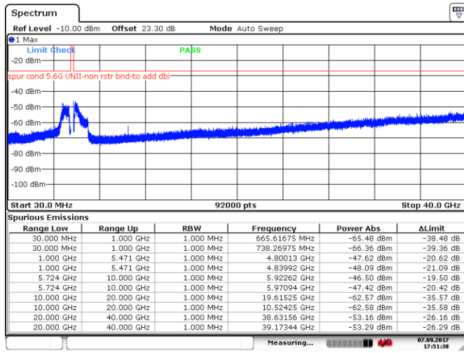
Figure 8.5-29: Spurious emissions outside restricted bands, 10 MHz channel, high channel, 24 dBi antenna, cho
