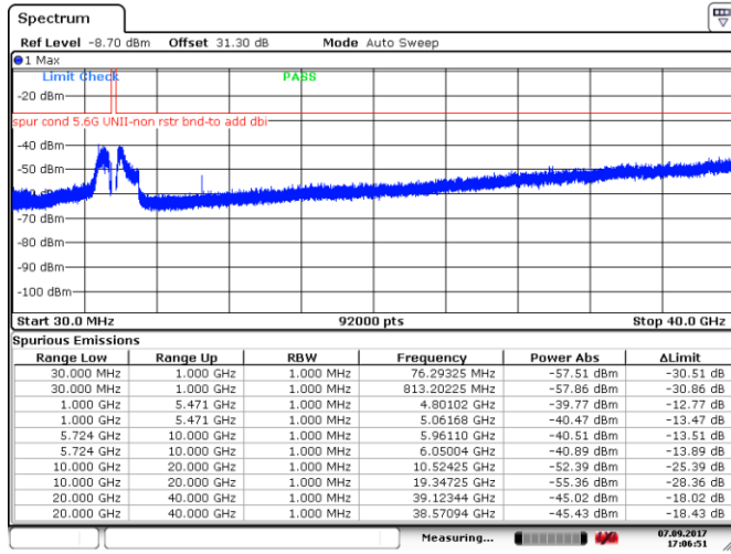
Figure 8.5-13: Spurious emissions outside restricted bands, 5 MHz channel, low channel, 32 dBi antenna, cho
