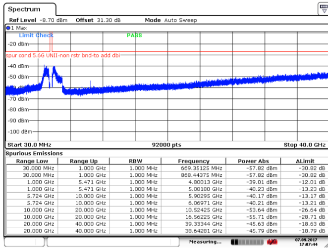
Figure 8.5-17: Spurious emissions outside restricted bands, 5 MHz channel, high channel, 32 dBi antenna, cho
