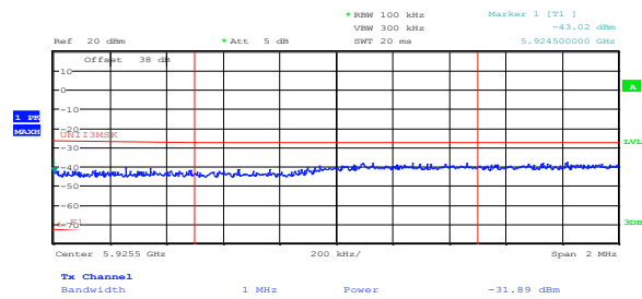
Figure 8.2-31: Conducted spurious emissions at the upper band edge at 5925 MHz, 5 MHz high channel, for 24 dBi antenna, ch1, PTP application
