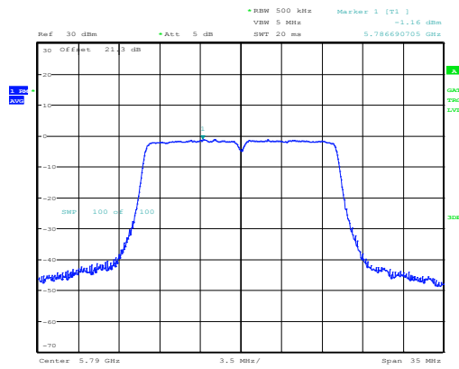
Figure 8.1-6: Sample plot for PSD on 20 MHz
