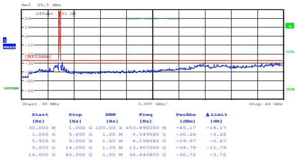
Figure 8.2-6: Conducted spurious emissions outside restricted bands, 5 MHz low channel, for 24 dBi antenna, ch1, PTP application
