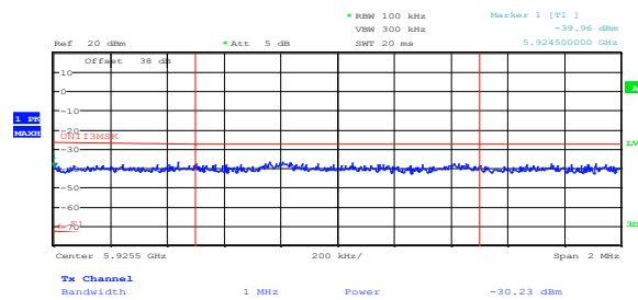
Figure 8.2-39: Conducted spurious emissions at the upper band edge at 5925 MHz, 20 MHz high channel, for 24 dBi antenna, ch1, PTP application
