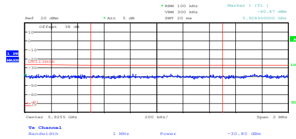
Figure 8.2-37: Conducted spurious emissions at the upper band edge at 5925 MHz, 20 MHz high channel, for 24 dBi antenna, ch0, PTP application
