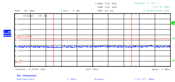
Figure 8.2-35: Conducted spurious emissions at the upper band edge at 5925 MHz, 10 MHz high channel, for 24 dBi antenna, ch1, PTP application
