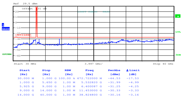
Figure 8.2-8: Conducted spurious emissions outside restricted bands, 10 MHz low channel, for 24 dBi antenna, cho, PTP application
