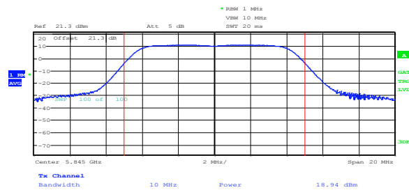
Figure 8.1-2: Sample plot for Power on 10 MHz
