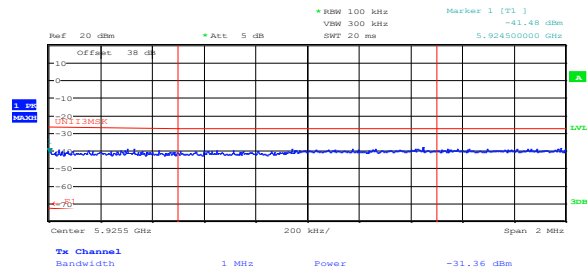
Figure 8.2-29: Conducted spurious emissions at the upper band edge at 5925 MHz, 5 MHz high channel, for 24 dBi antenna, cho, PTP application
