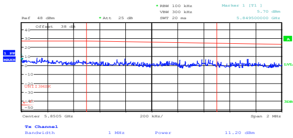
Figure 8.2-36: Conducted spurious emissions at the upper band edge at 5850 MHz, 20 MHz high channel, for 24 dBi antenna, ch0, PTP application
