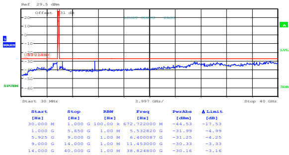
Figure 8.2-10: Conducted spurious emissions outside restricted bands, 10 MHz low channel, for 24 dBi antenna, ch1, PTP application
