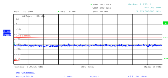
Figure 8.2-33: Conducted spurious emissions at the upper band edge at 5925 MHz, 10 MHz high channel, for 24 dBi antenna, cho, PTP application
