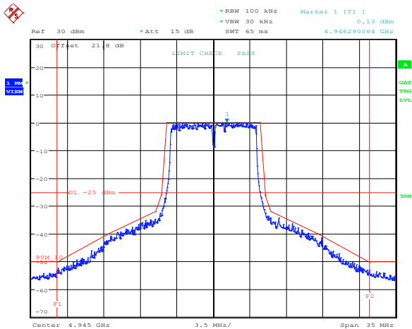
Figure 8.6-18: Emission mask for 10 MHz channel, antenna port 2, low frequency, BPSK
