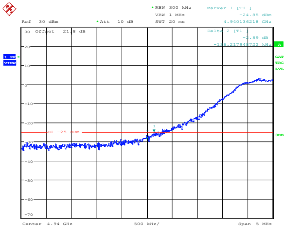
Figure 8.8-3: Lower band edge for 10 MHz channel, low frequency ( f_L )
