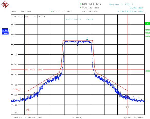
Figure 8.6-2: Emission mask for 5 MHz channel, antenna port 1, low frequency, BPSK
