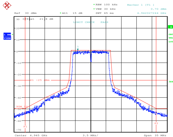
Figure 8.6-19: Emission mask for 10 MHz channel, antenna port 2, low frequency, QPSK
