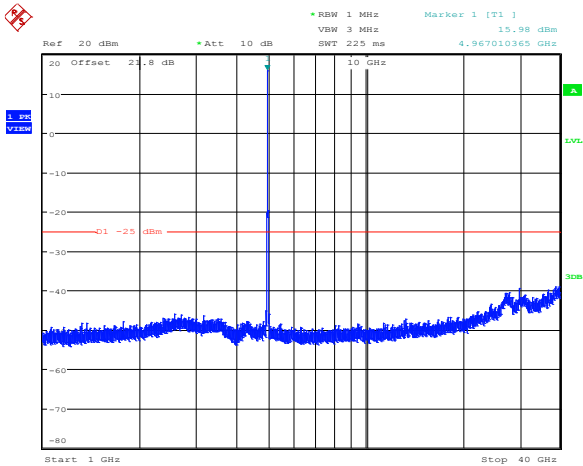
Figure 8.6-94: Spurious emissions sample plot above 1 GHz, antenna port 1, 20 MHz channel, BPSK
