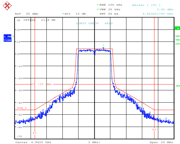
Figure 8.6-3: Emission mask for 5 MHz channel, antenna port 1, low frequency, QPSK
