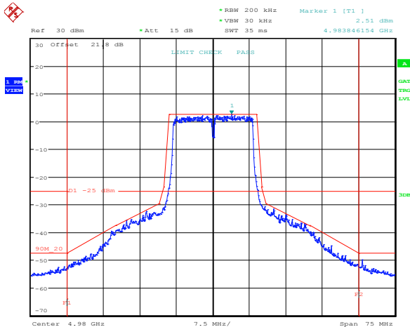
Figure 8.6-58: Emission mask for 20 MHz channel, antenna port 1, high frequency, BPSK
