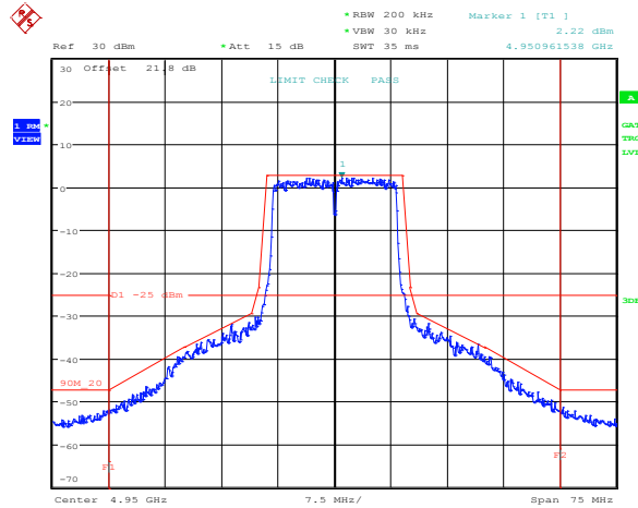
Figure 8.6-23: Emission mask for 20 MHz channel, antenna port 2, low frequency, QPSK
