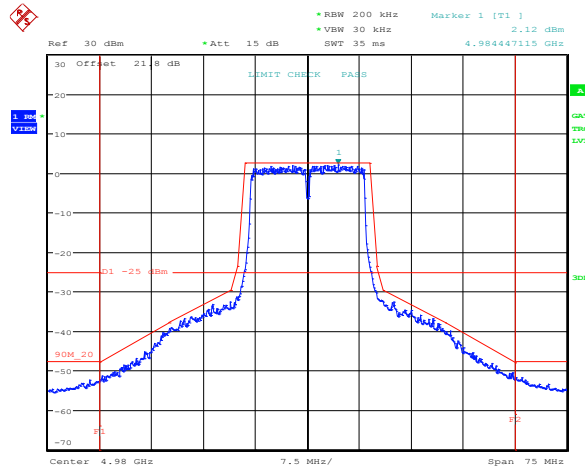
Figure 8.6-71: Emission mask for 20 MHz channel, antenna port 2, high frequency, QPSK
