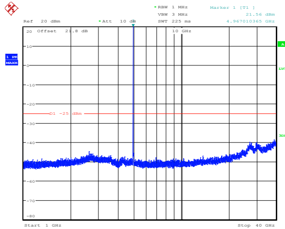
Figure 8.6-87: Spurious emissions sample plot above 1 GHz, antenna port 2, 5 MHz channel, BPSK
