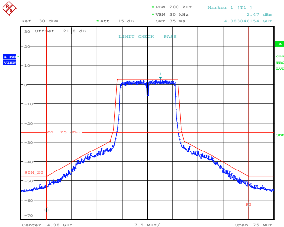
Figure 8.6-70: Emission mask for 20 MHz channel, antenna port 2, high frequency, BPSK
