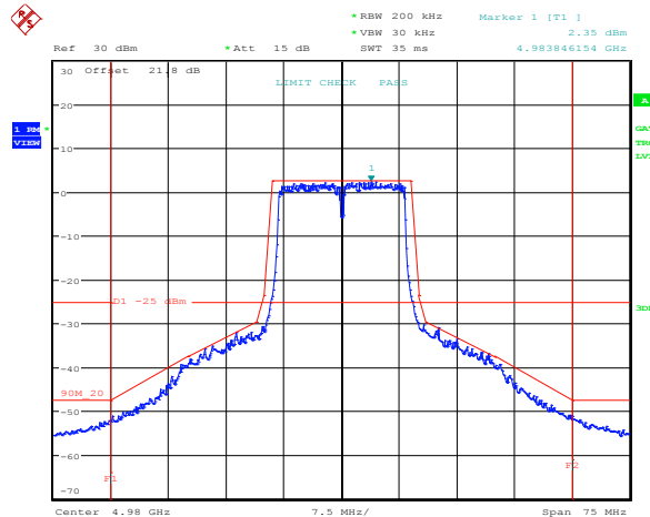
Figure 8.6-59: Emission mask for 20 MHz channel, antenna port 1, high frequency, QPSK
