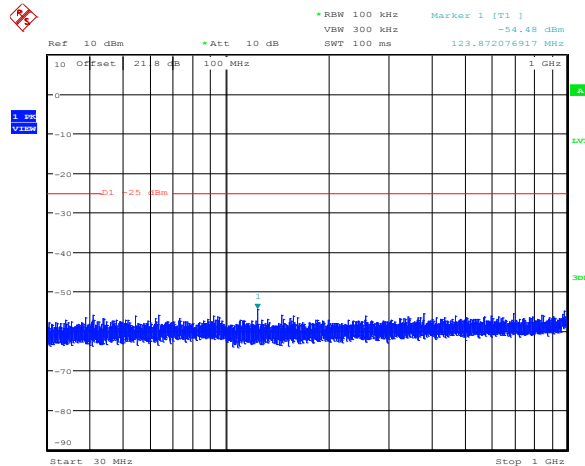
Figure 8.6-75: Spurious emissions sample plot below 1 GHz, antenna port 2, 5 MHz channel, BPSK
