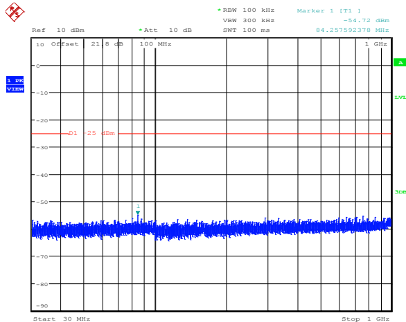
Figure 8.6-74: Spurious emissions sample plot below 1 GHz, antenna port 1, 5 MHz channel, BPSK
