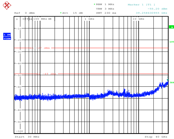
Diagram 8.5-81: Conducted spurious emissions for IC, 19 dBi antenna, 5 MHz channel, ch1, low frequency
