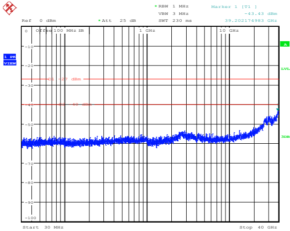
Diagram 8.5-10: Conducted spurious emissions for FCC, 10 dBi antenna, 5 MHz channel, ch1, mid frequency
