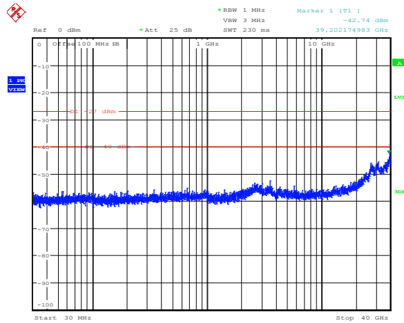
Diagram 8.5-15: Conducted spurious emissions for FCC, 10 dBi antenna, 10 MHz channel, ch1, low frequency
