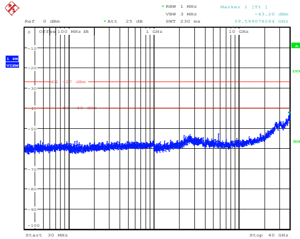
Diagram 8.5-61: Conducted spurious emissions for IC, 10 dBi antenna, 5 MHz channel, cho, mid frequency
