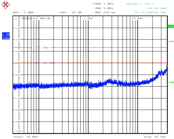
Diagram 8.5-60: Conducted spurious emissions for IC, 10 dBi antenna, 5 MHz channel, cho, low frequency
