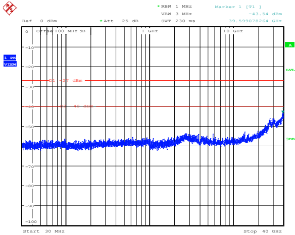
Diagram 8.5-64: Conducted spurious emissions for IC, 10 dBi antenna, 5 MHz channel, ch1, mid frequency
