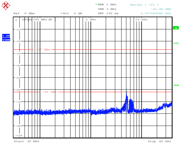
Diagram 8.5-46: Conducted spurious emissions for FCC, 32 dBi antenna, 5 MHz channel, ch1, mid frequency
