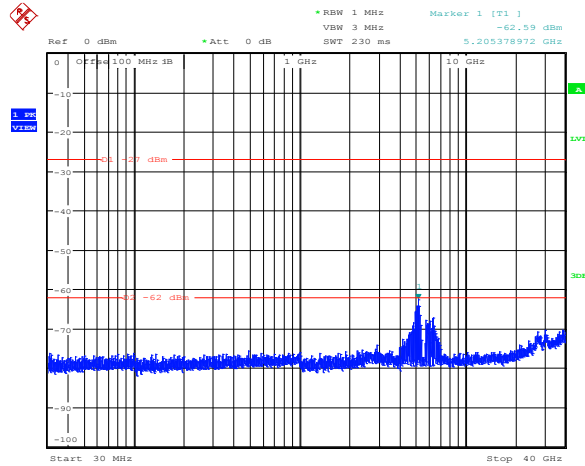
Diagram 8.5-43: Conducted spurious emissions for FCC, 32 dBi antenna, 5 MHz channel, cho, mid frequency
