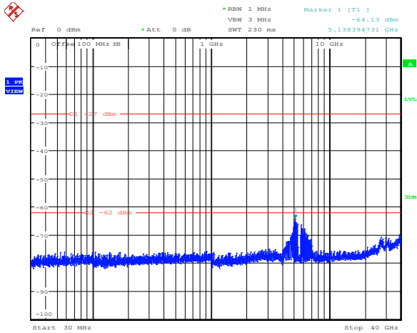
Diagram 8.5-108: Conducted spurious emissions for IC, 32 dBi antenna, 20 MHz channel, cho, low frequency
