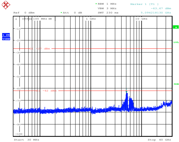
Diagram 8.5-42: Conducted spurious emissions for FCC, 32 dBi antenna, 5 MHz channel, cho, low frequency
