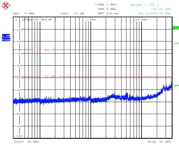
Diagram 8.5-80: Conducted spurious emissions for IC, 19 dBi antenna, 5 MHz channel, cho, high frequency
