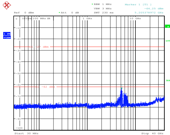
Diagram 8.5-47: Conducted spurious emissions for FCC, 32 dBi antenna, 5 MHz channel, ch1, high frequency
