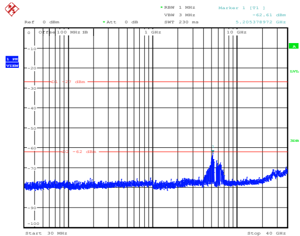
Diagram 8.5-51: Conducted spurious emissions for FCC, 32 dBi antenna, 10 MHz channel, ch1, low frequency
