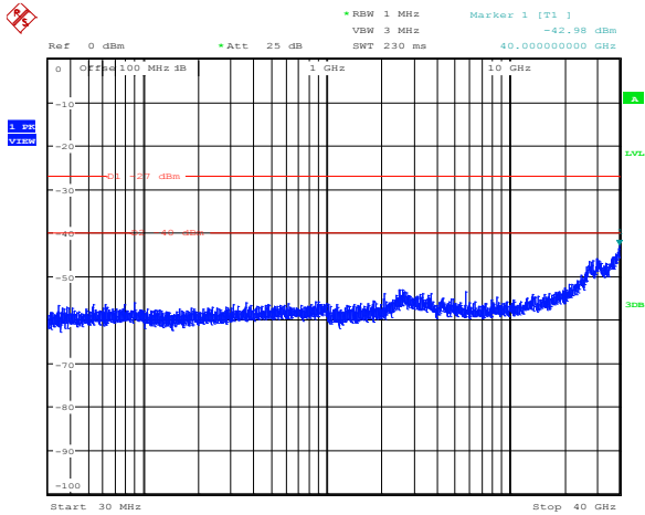
Diagram 8.5-6: Conducted spurious emissions for FCC, 10 dBi antenna, 5 MHz channel, cho, low frequency
