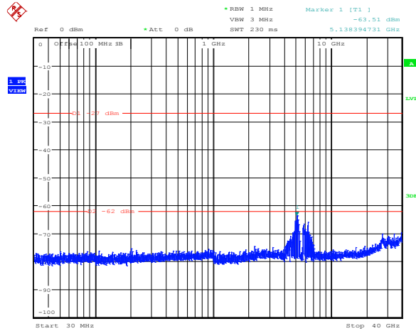
Diagram 8.5-97: Conducted spurious emissions for IC, 32 dBi antenna, 5 MHz channel, cho, mid frequency
