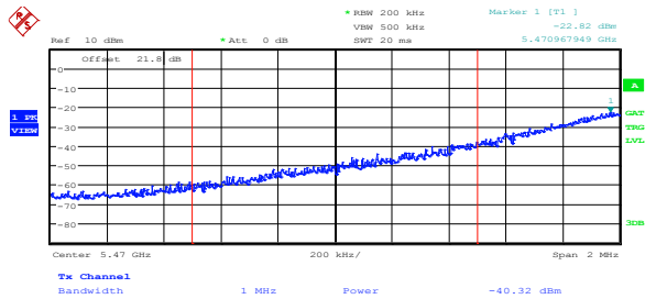
Diagram 8.5-4: Lower band edge sample plot
