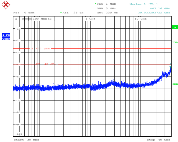
Diagram 8.5-72: Conducted spurious emissions for IC, 10 dBi antenna, 20 MHz channel, cho, low frequency
