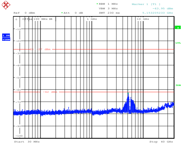
Diagram 8.5-96: Conducted spurious emissions for IC, 32 dBi antenna, 5 MHz channel, cho, low frequency
