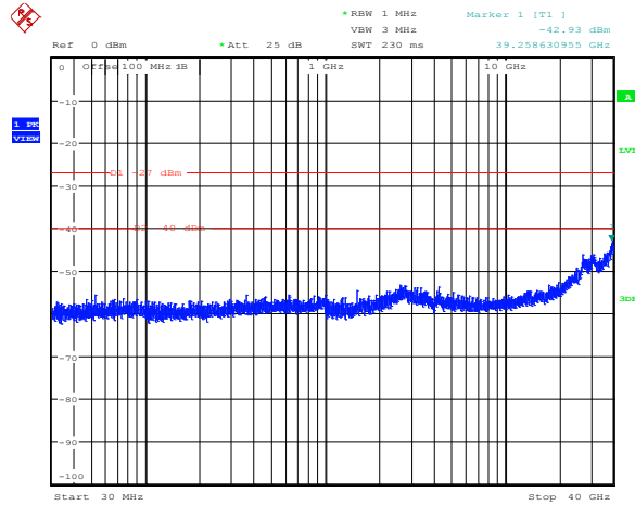
Diagram 8.5-7: Conducted spurious emissions for FCC, 10 dBi antenna, 5 MHz channel, cho, mid frequency
