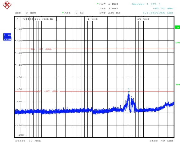
Diagram 8.5-109: Conducted spurious emissions for IC, 32 dBi antenna, 20 MHz channel, cho, mid frequency
