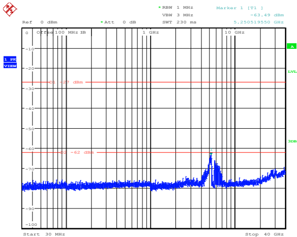
Diagram 8.5-50: Conducted spurious emissions for FCC, 32 dBi antenna, 10 MHz channel, cho, high frequency
