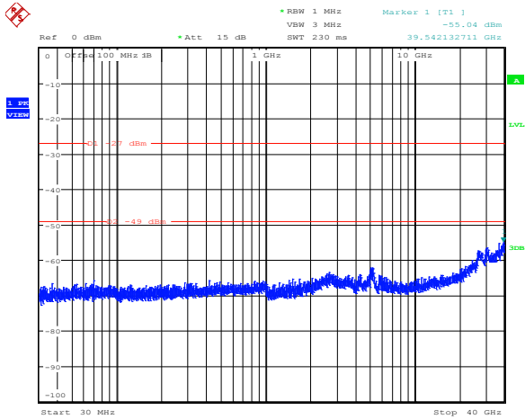
Diagram 8.5-34: Conducted spurious emissions for FCC, 19 dBi antenna, 10 MHz channel, ch1, mid frequency
