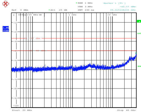
Diagram 8.5-69: Conducted spurious emissions for IC, 10 dBi antenna, 10 MHz channel, ch1, low frequency
