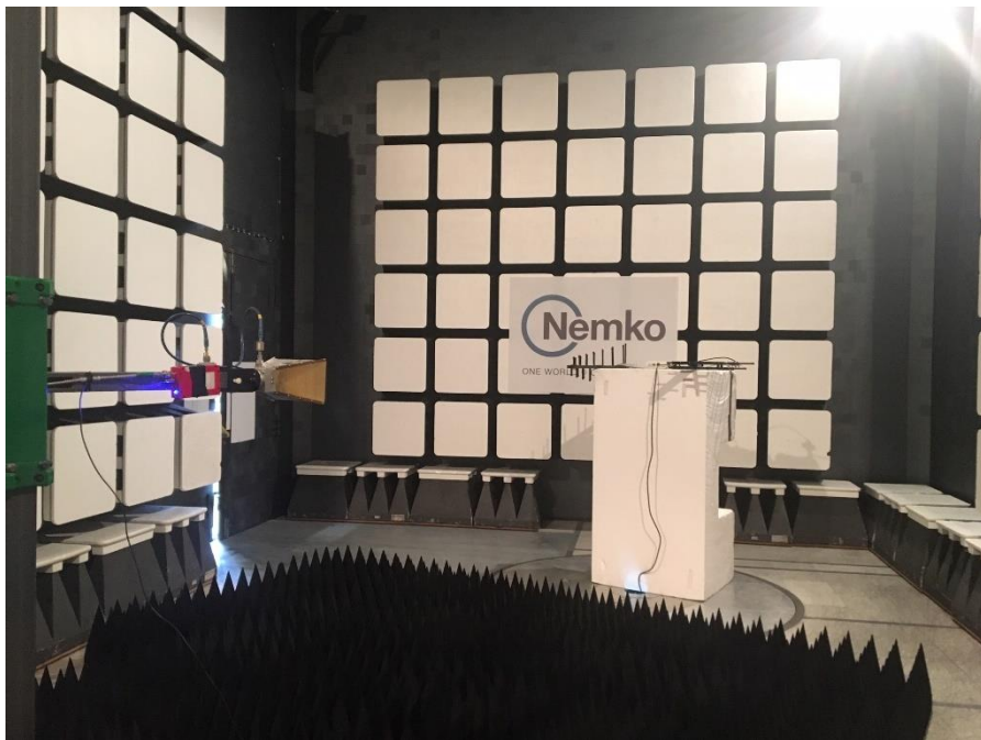
Radiated spurious emissions above 1 GHz with Log-P antenna
