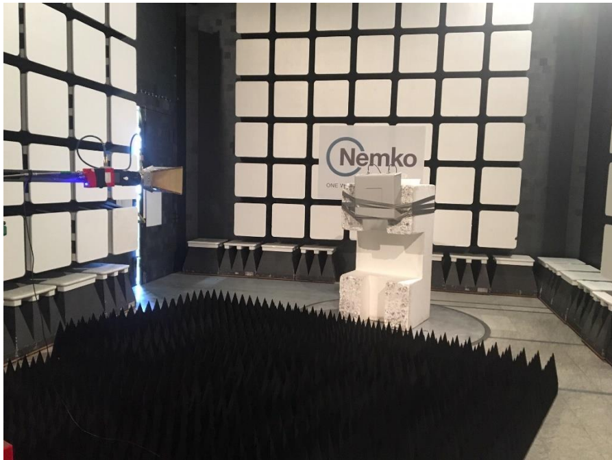
Radiated spurious emissions above 1 GHz with Flat antenna
