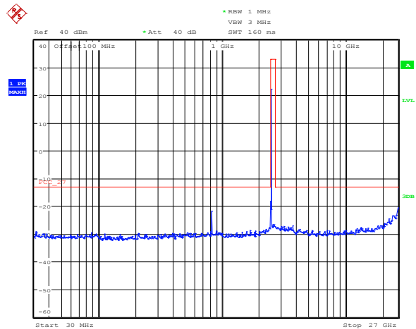
Figure 8.2-24: Conducted spurious emissions at antenna port 2, high channel, 5 MHz BW, 256-QAM
