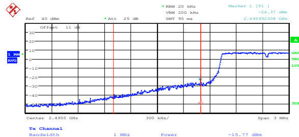
Figure 8.2-34: Conducted lower band edge emissions at antenna port 2, 1.25 MHz BW, BPSK
