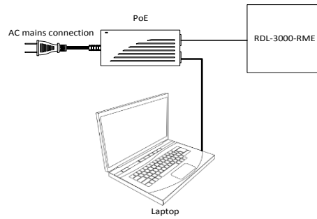
Figure 3.6-1: Setup diagram
