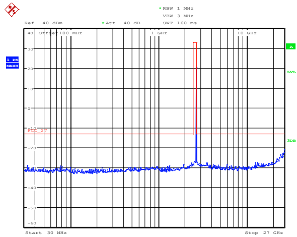
Figure 8.2-28: Conducted spurious emissions at antenna port 2, low channel, 10 MHz BW, 256-QAM
