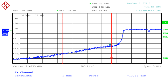
Figure 8.2-33: Conducted lower band edge emissions at antenna port 1, 1.25 MHz BW, BPSK
