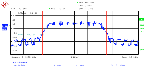
Figure 8.1-3: Output power for 5 MHz channel BW, sample plot
