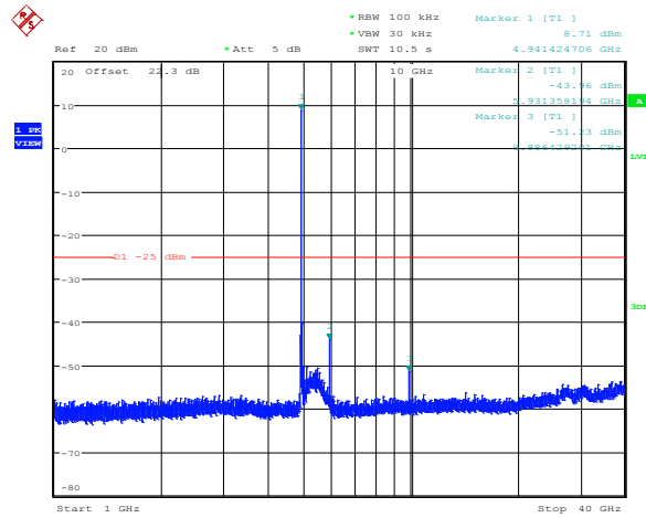
Plot 8.5-87: Spurious emissions above 1 GHz for 5 MHz channel, antenna port 2, low frequency, 16-QAM
