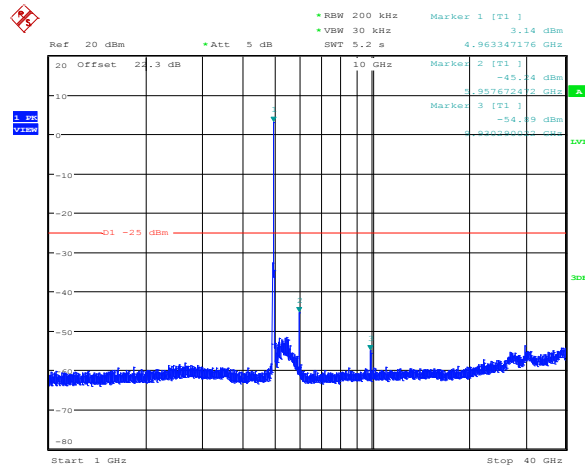
Plot 8.5-167: Spurious emissions above 1 GHz for 20 MHz channel, antenna port 2, mid frequency, 16-QAM
