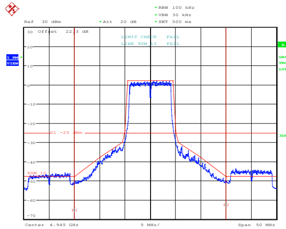
Plot 8.5-7: Emission mask for 10 MHz channel, antenna port 1, low frequency, QPSK
