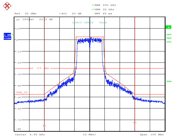
Plot 8.5-11: Emission mask for 20 MHz channel, antenna port 1, low frequency, QPSK
