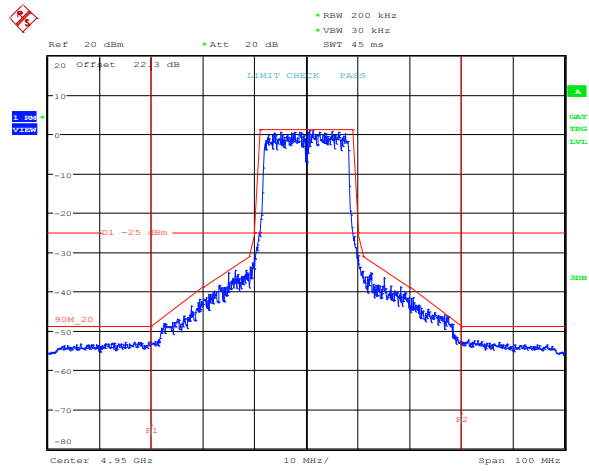
Plot 8.5-23: Emission mask for 20 MHz channel, antenna port 2, low frequency, QPSK
