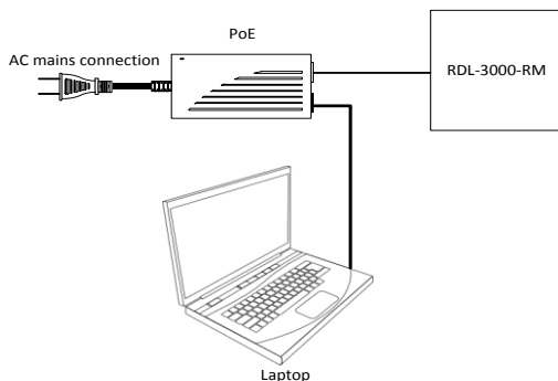
Diagram 3.6-1: Setup diagram
