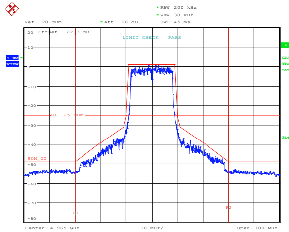
Plot 8.5-47: Emission mask for 20 MHz channel, antenna port 2, mid frequency, QPSK
