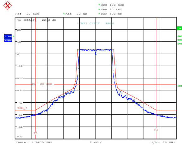
Plot 8.5-51: Emission mask for 5 MHz channel, antenna port 1, high frequency, QPSK
