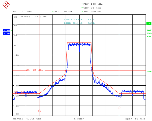
Plot 8.5-31: Emission mask for 10 MHz channel, antenna port 1, mid frequency, QPSK
