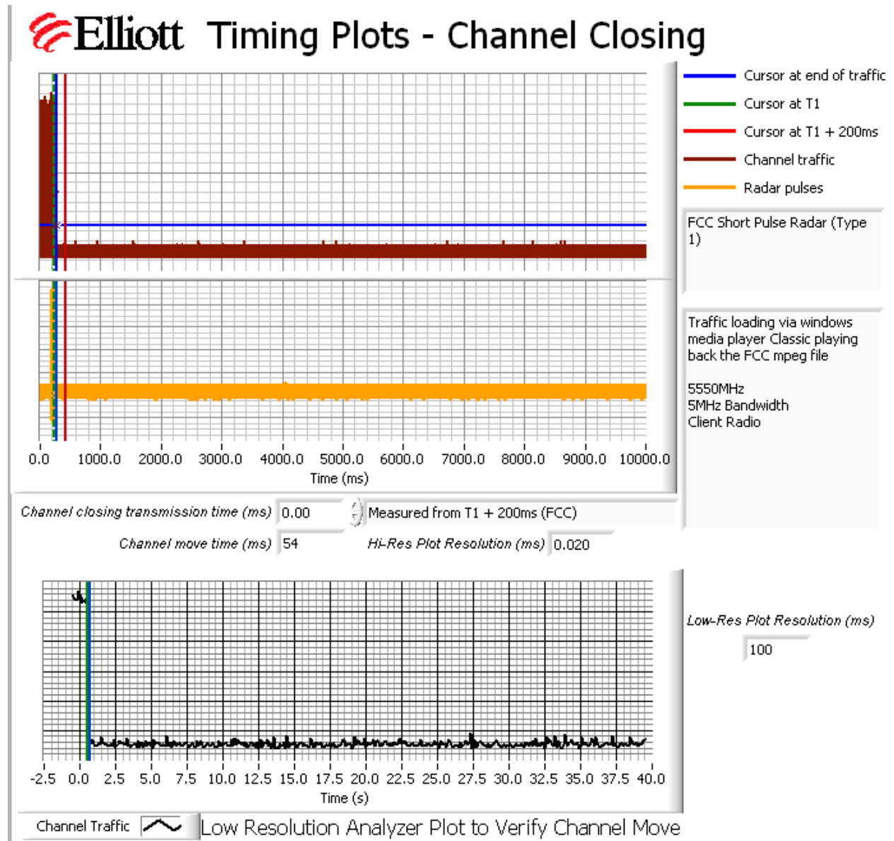
Figure 3 Channel Closing Time and Channel Move Time – 40 second plot, 5MHz Bandwidth
