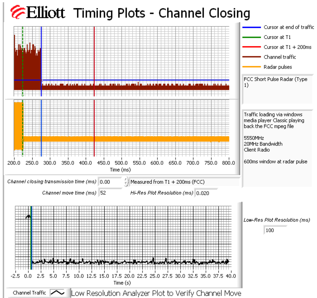
Figure 8 Close-Up of Transmissions Occurring More Than 200ms After The End of Radar
