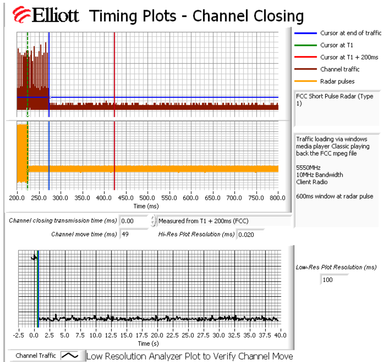
Figure 6 Close-Up of Transmissions Occurring More Than 200ms After The End of Radar, 10MHz BW
