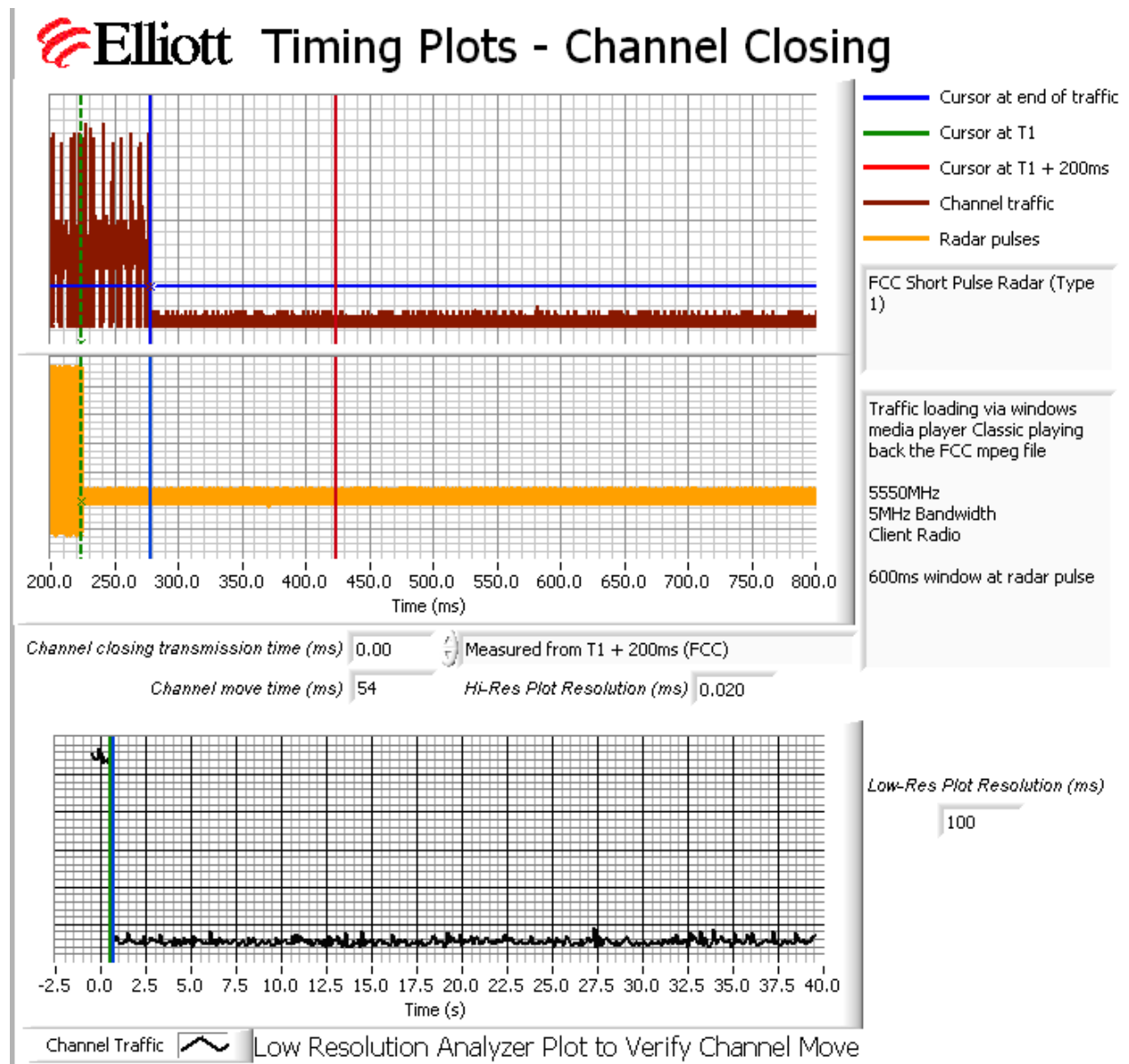
Figure 4 Close-Up of Transmissions Occurring More Than 200ms After The End of Radar, 5MHz BW
