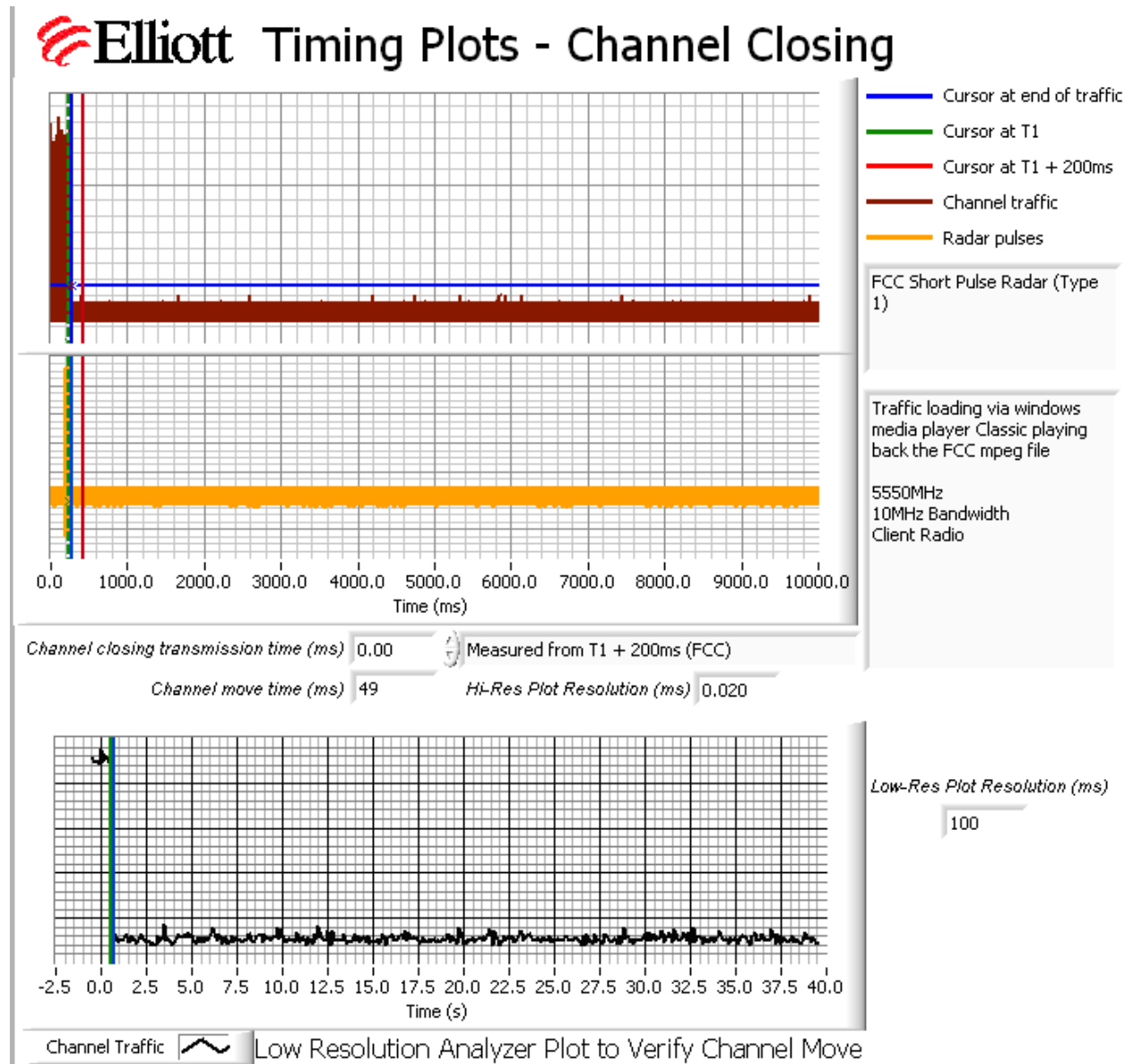
Figure 5 Channel Closing Time and Channel Move Time – 40 second plot, 10MHz Bandwidth
