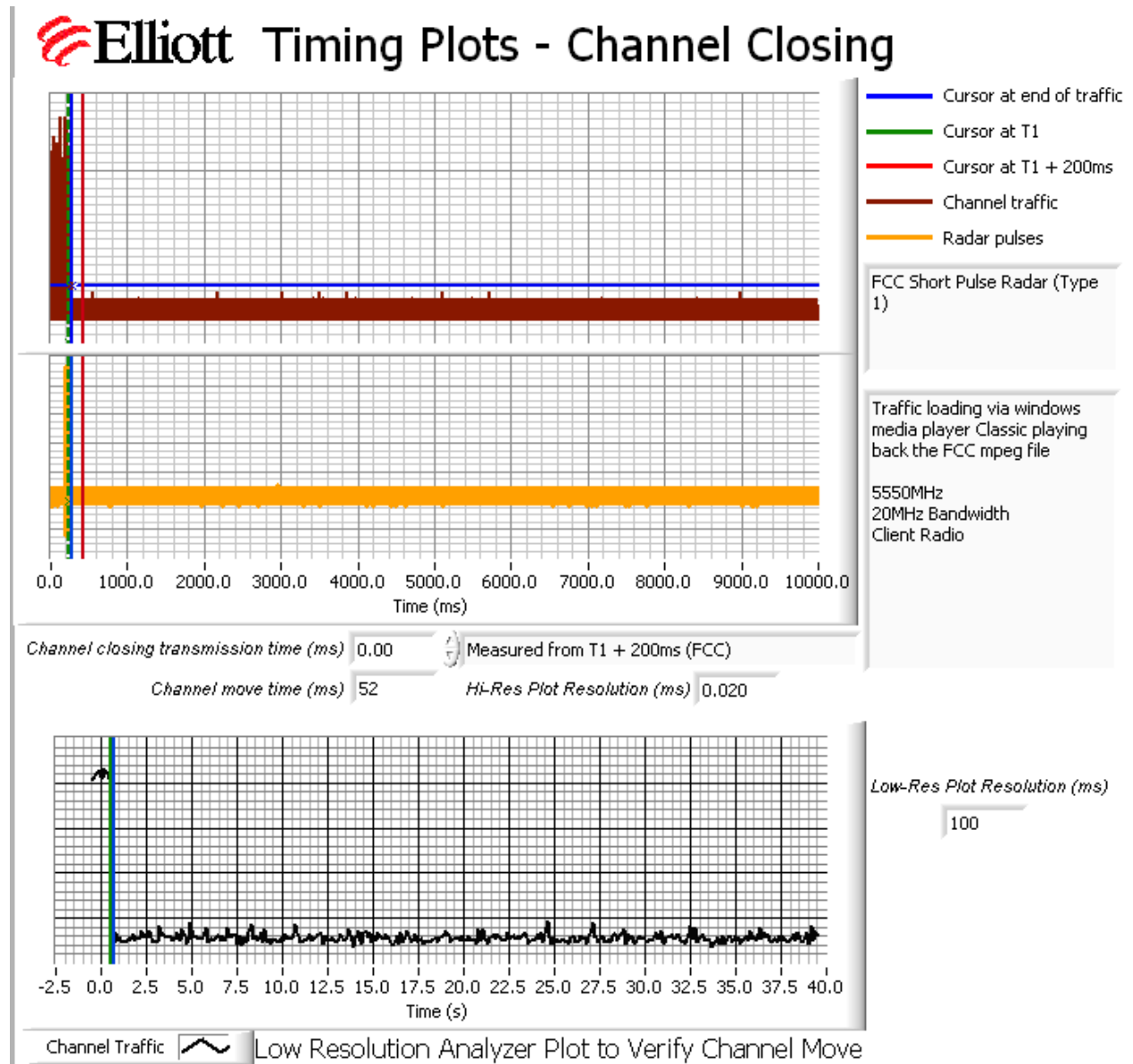
Figure 7 Channel Closing Time and Channel Move Time – 40 second plot, 20MHz Bandwidth
