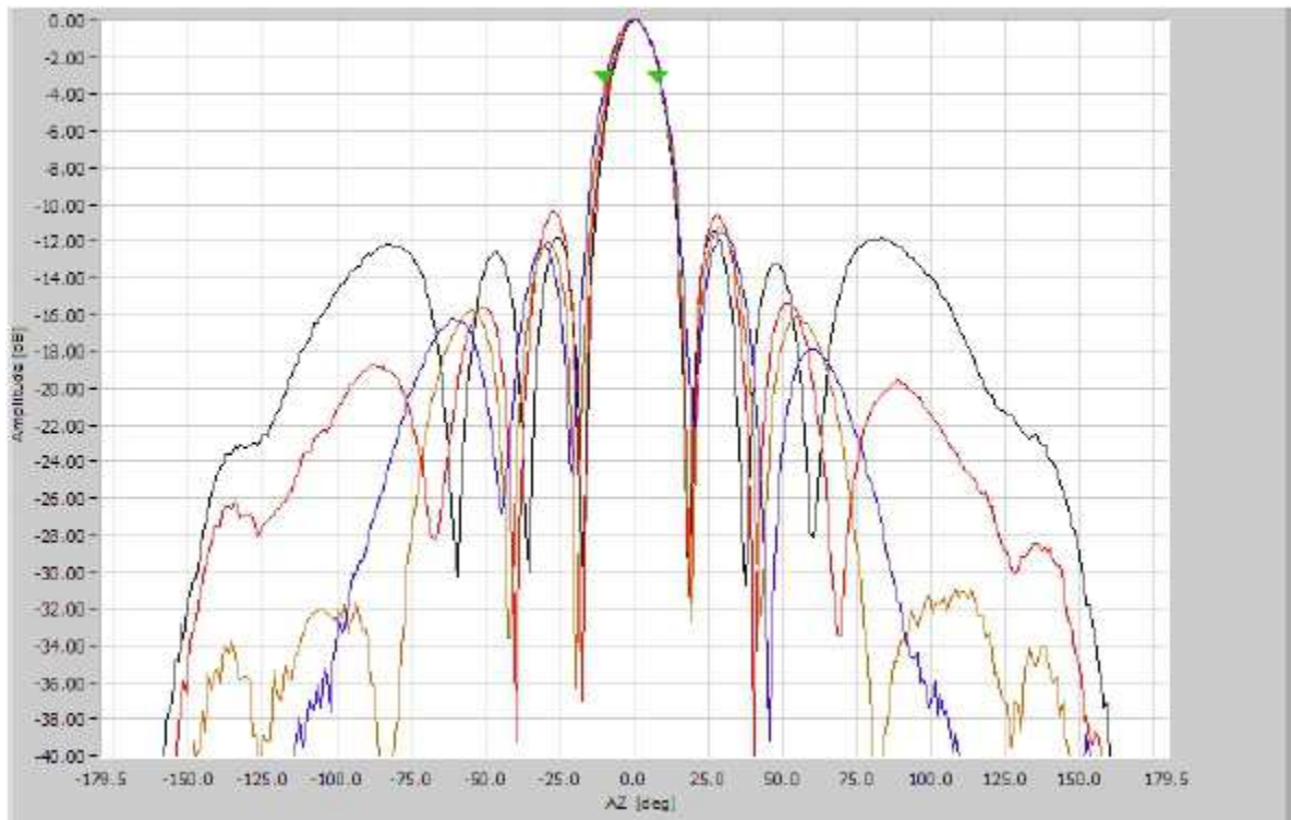
Horizontal Polarization – Azimuth (e-plane)
