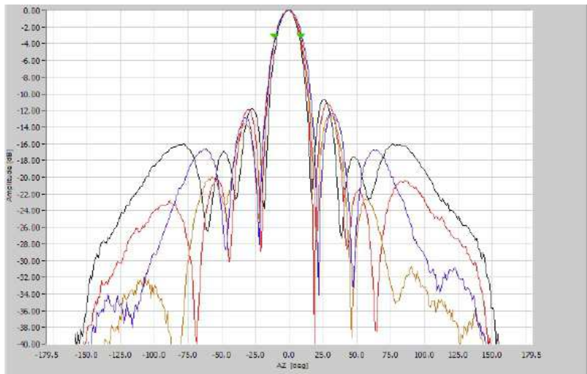
Vertical Polarization – Azimuth (h-plane)
