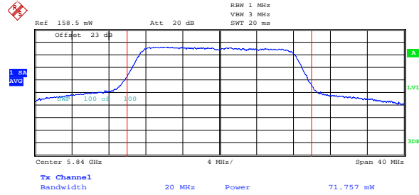
Antenna Port 2
