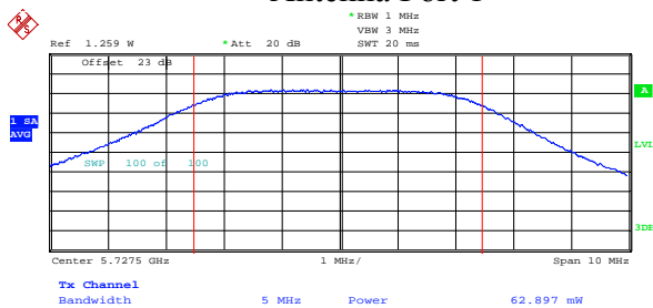
Antenna Port 1
