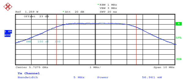
Antenna Port 2
