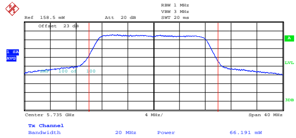
Antenna Port 2
