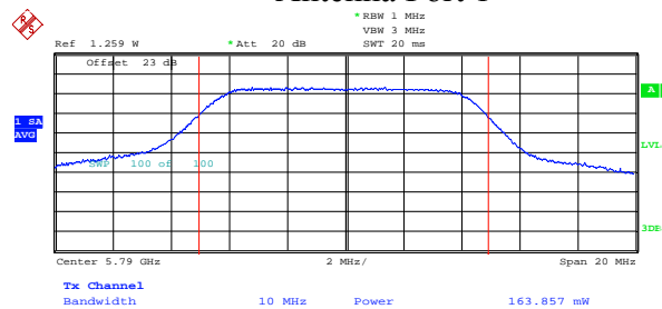
Antenna Port 1
