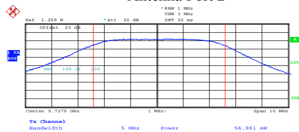
Antenna Port 2
