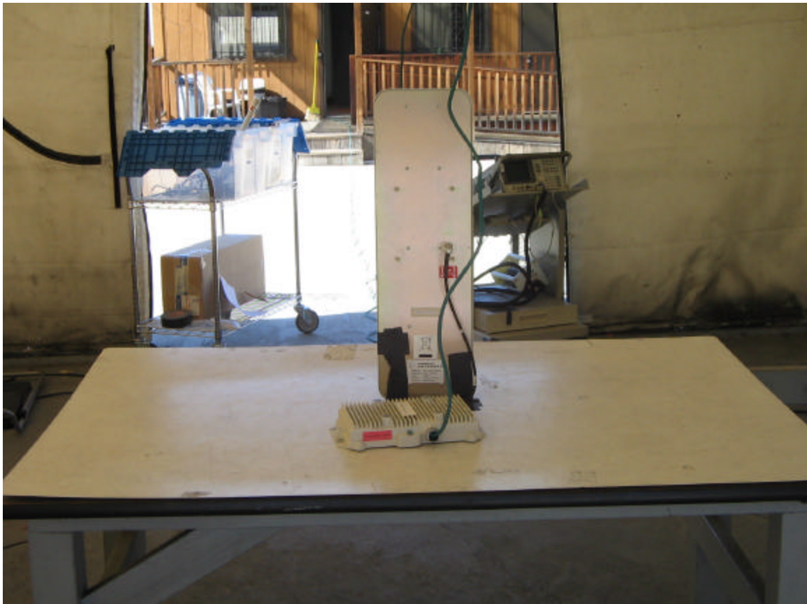
17.5dBi Sector antenna
