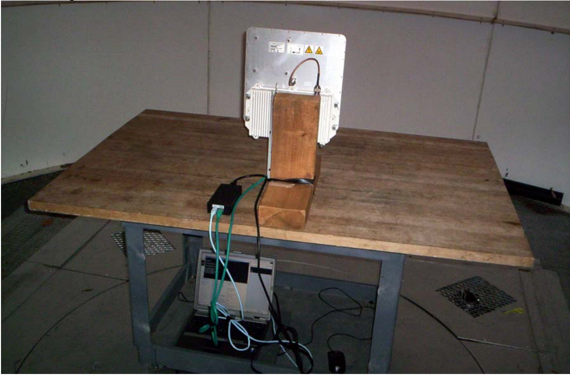
Radiated Spurious Emissions (OATS)
