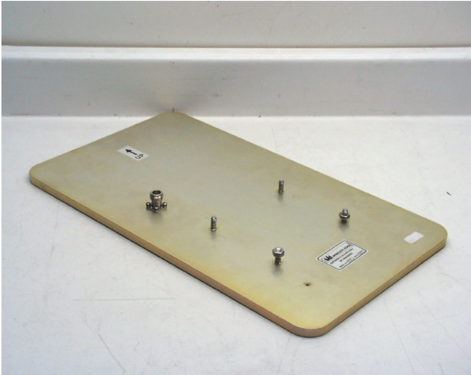
MTI Wireless Edge Antenna, P/N: 484026, Gain: 15 dBi (Back)
