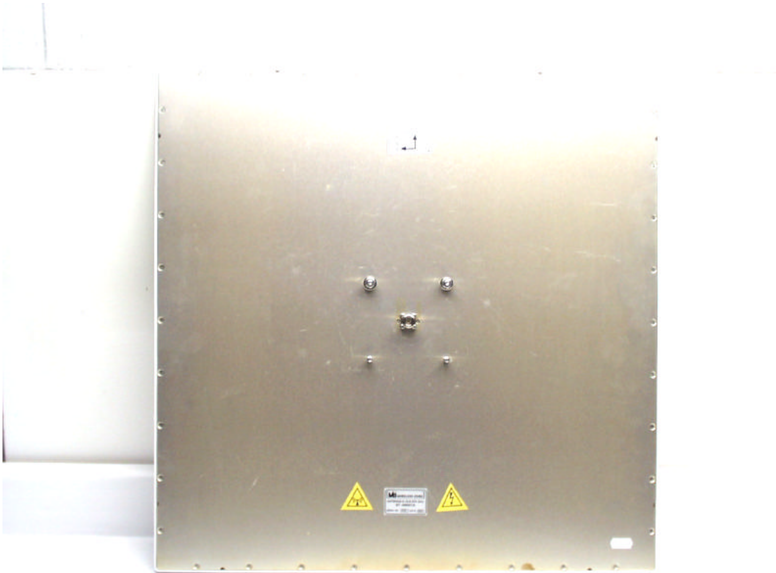
MTI Wireless Edge Antenna, P/N: 486001, Gain: 28 dBi (Back)
