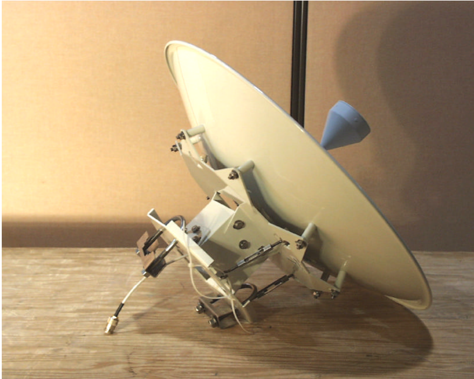
MaxRad Antenna P/N: MPR58029PT, Gain: 29 dBi (Back)
