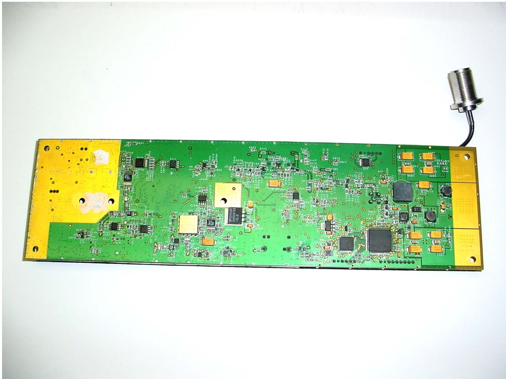
Out-door Unit
