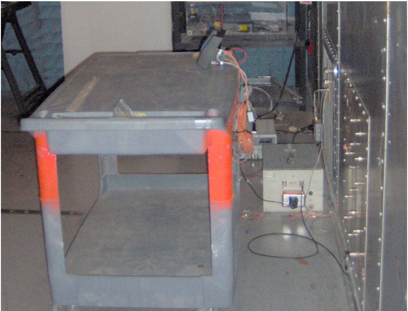
Power Lines Conducted Emissions (side view)
