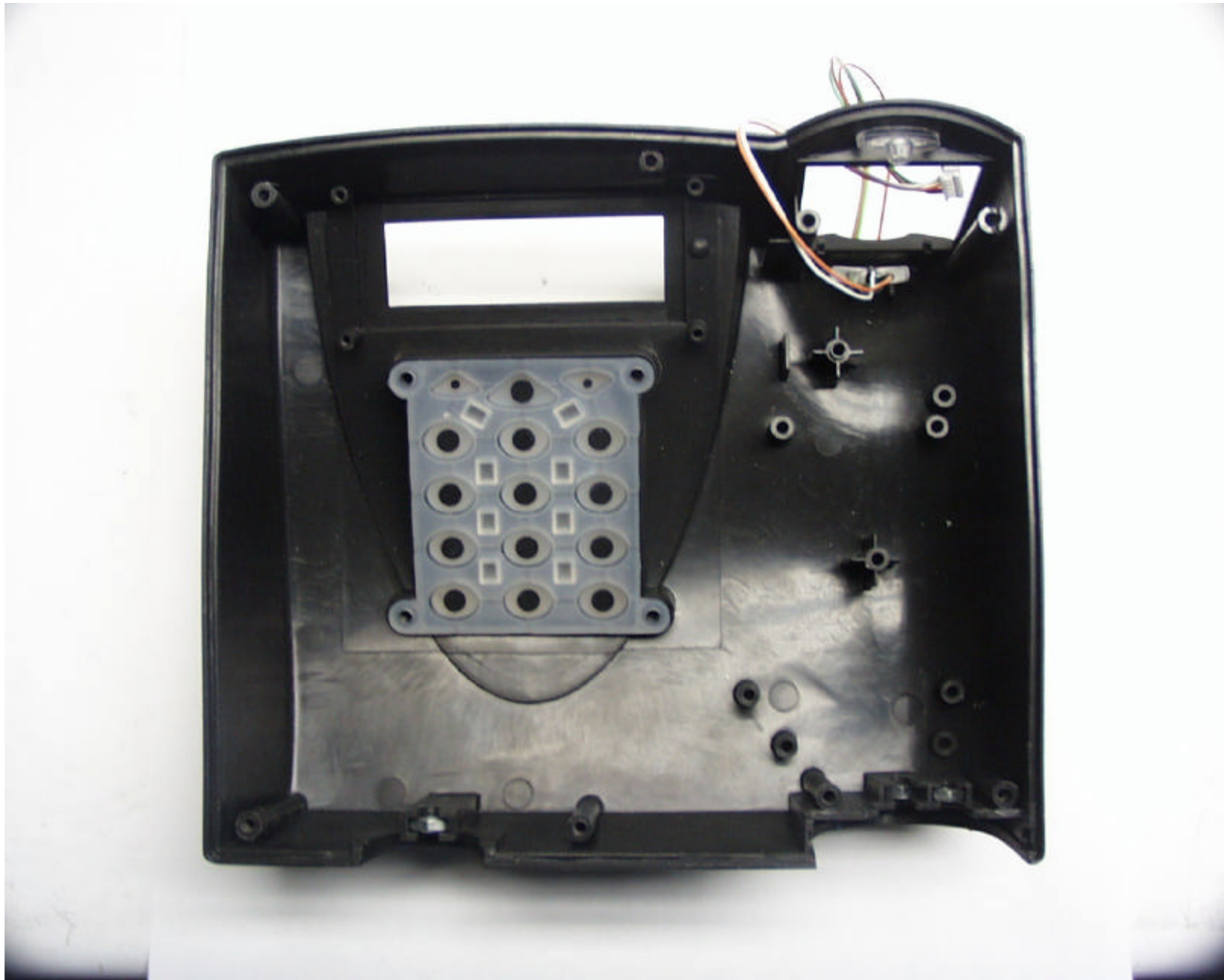
Annex 3 - Internal Photographs of Bioscrypt V-Station, A, H V-STATION, Model V-STATION, A, H
