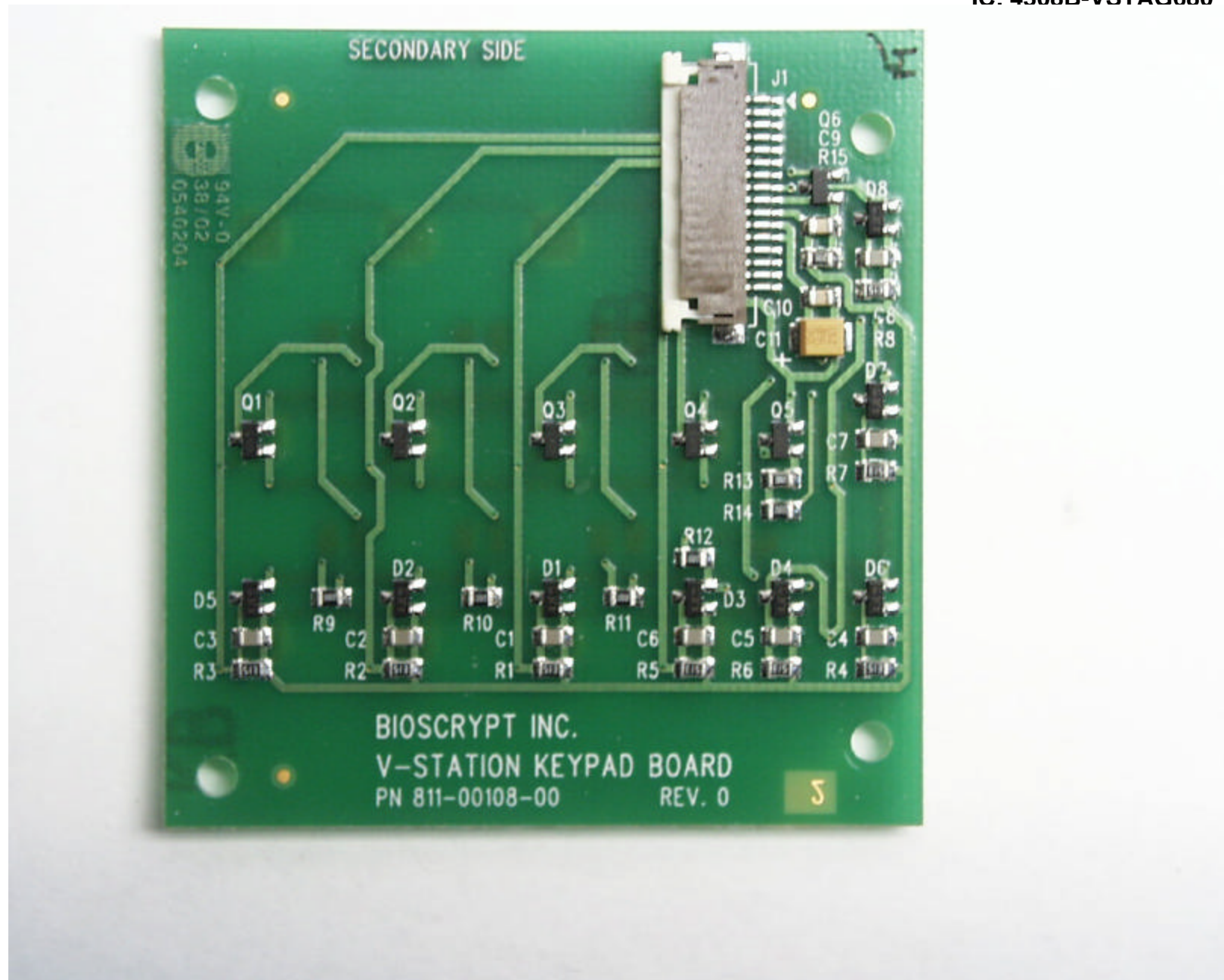
Photo # 7 FCC ID: QC4-VSTAG680 IC: 4308B-VSTAG680
