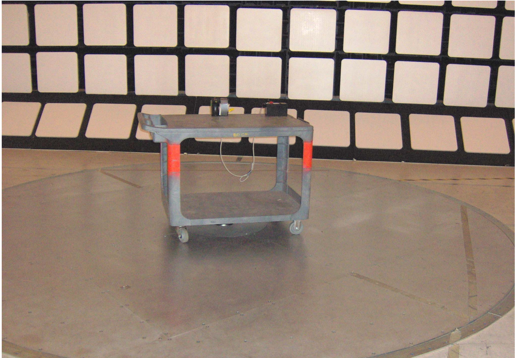
Photo #4: Radiated Emissions Measurements
