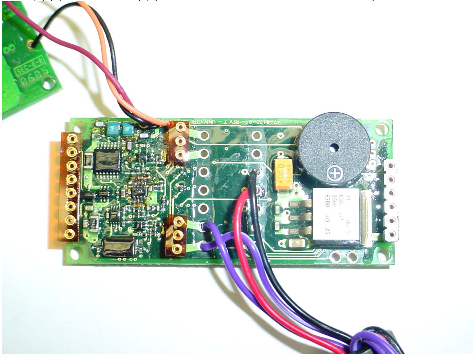
Annex 3: Internal Photographs of Device Under Test V-Smrt,A,H,R; Model No.: V-Smrt,A,H,R
