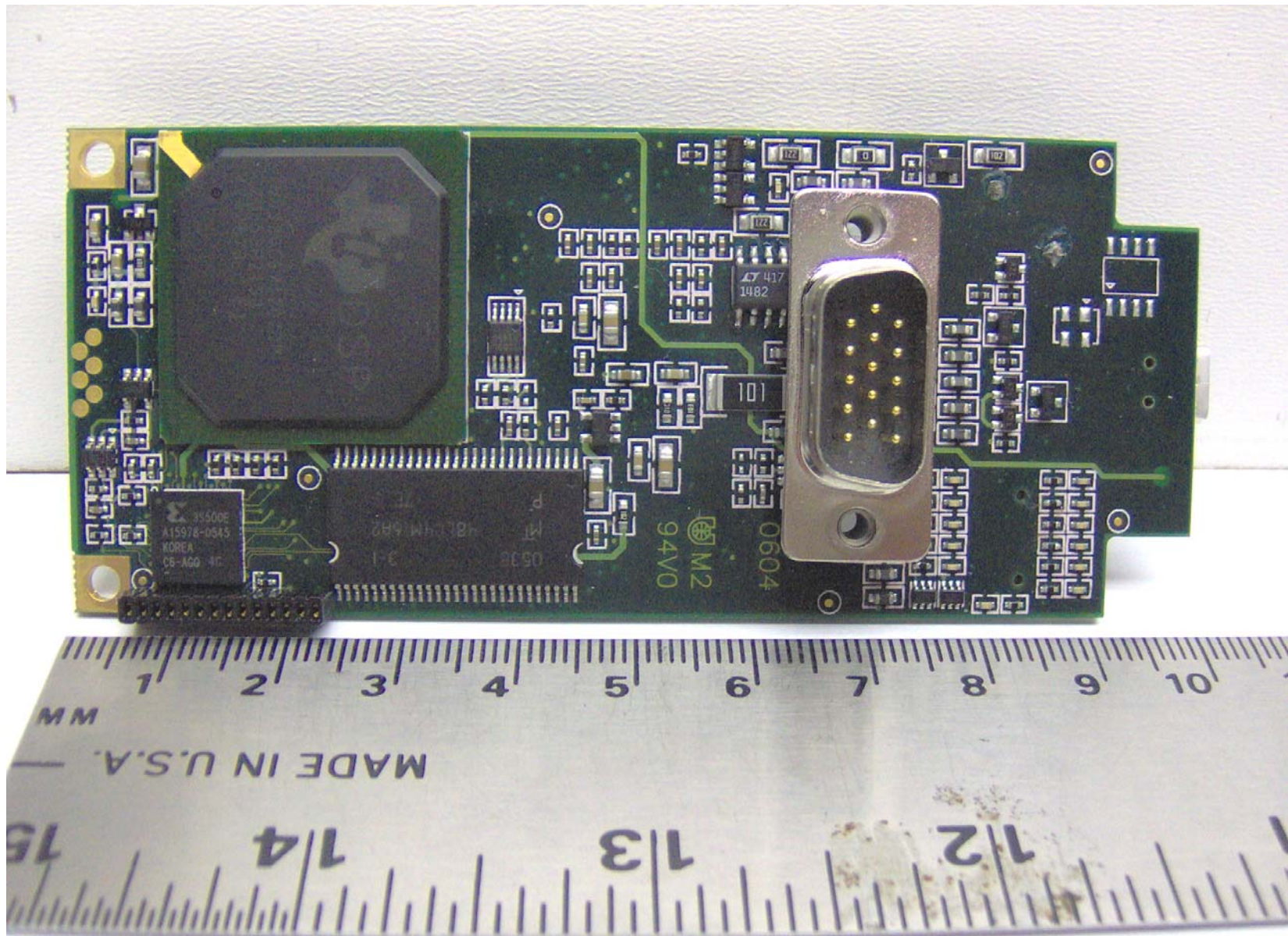
Annex 3: Internal Photographs of Device Under Test V-Smart,A,H,R; Model No.: V-Smrt,A,H,R
