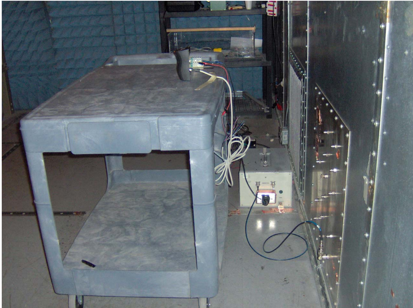
Photo #2: Powerline Conducted Emission Measurements
