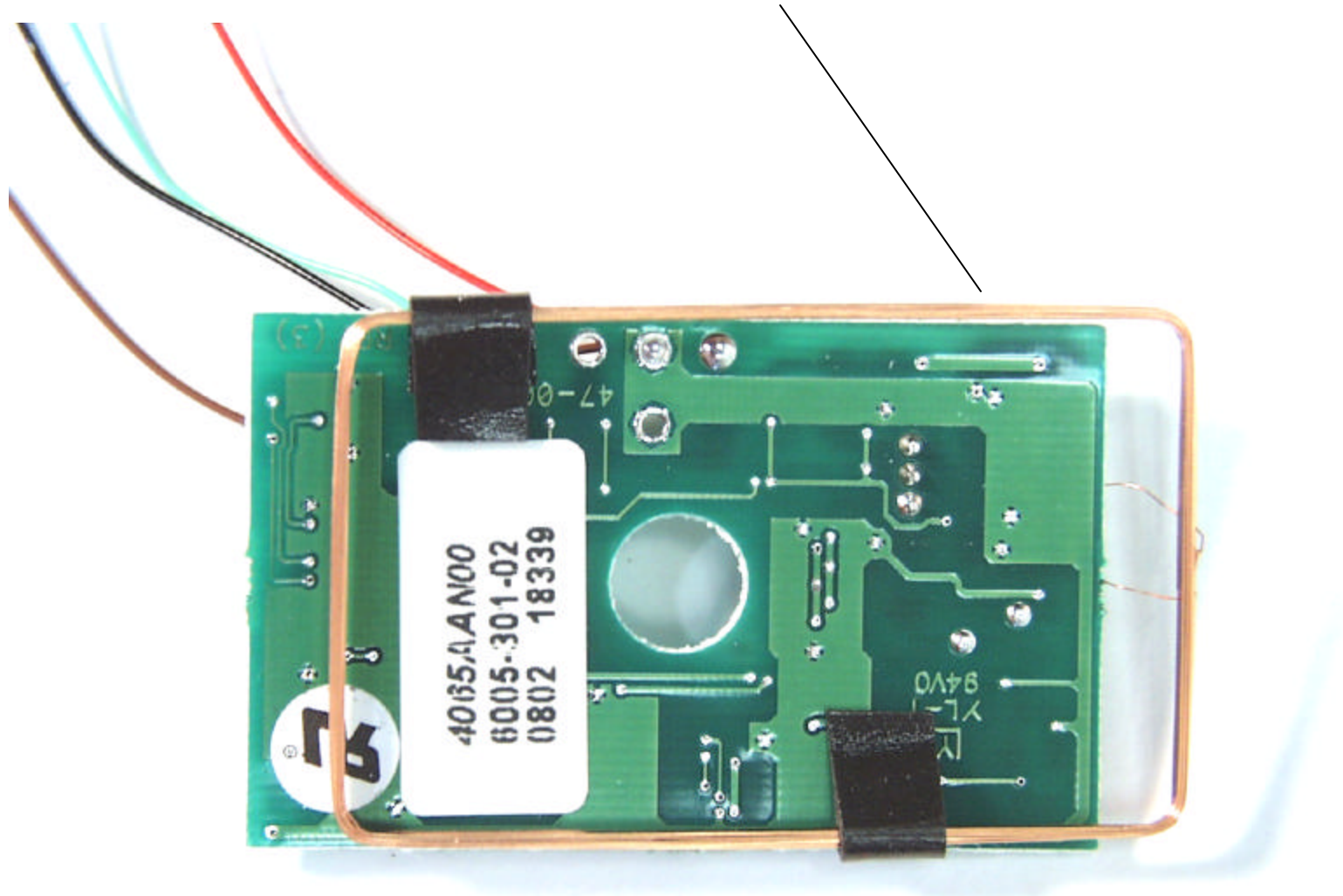
Proxy 125 KHz Radio Module with Integrated Loop Antenna (back)
