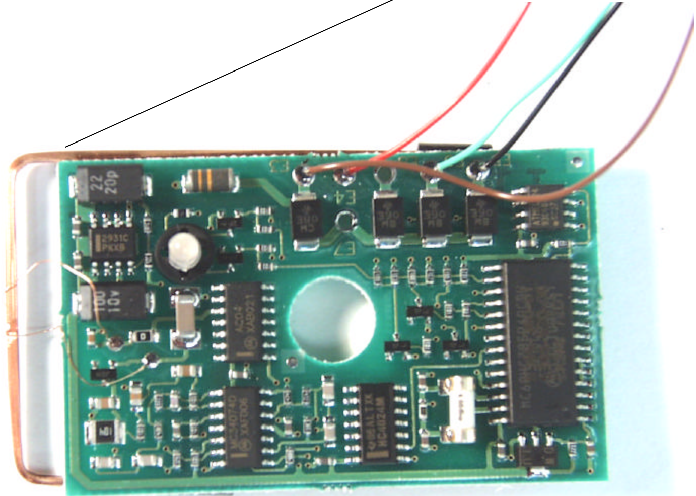
Proxy 125 KHz Radio Module with Integrated Loop Antenna (front)
