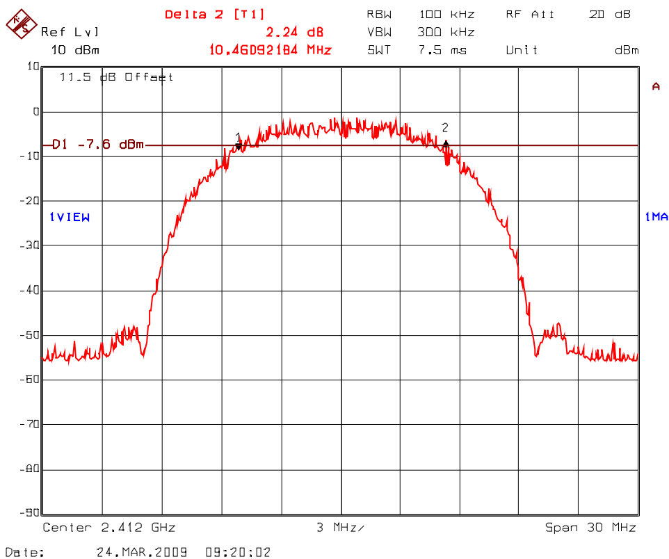
Plot 5.5.4.7. 6 dB Bandwidth Frequency: 2412 MHz; Modulation: CCK at 11 Mbps
