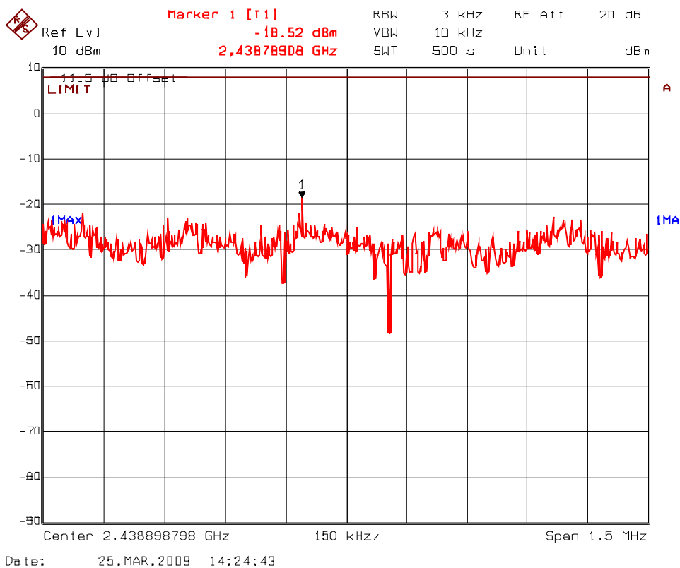
Plot 5.9.4.5. Power Spectral Density Frequency: 2437 MHz
