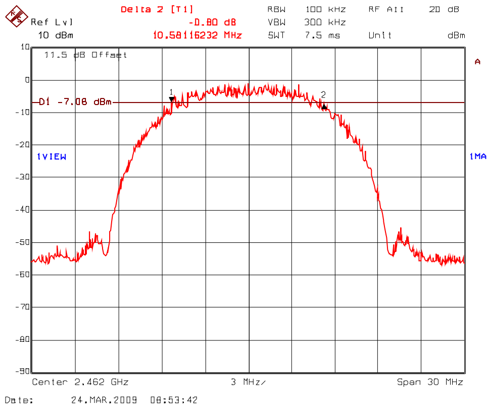
Plot 5.5.4.3. 6 dB Bandwidth Frequency: 2462 MHz; Modulation: DBPSK at 1 Mbps
