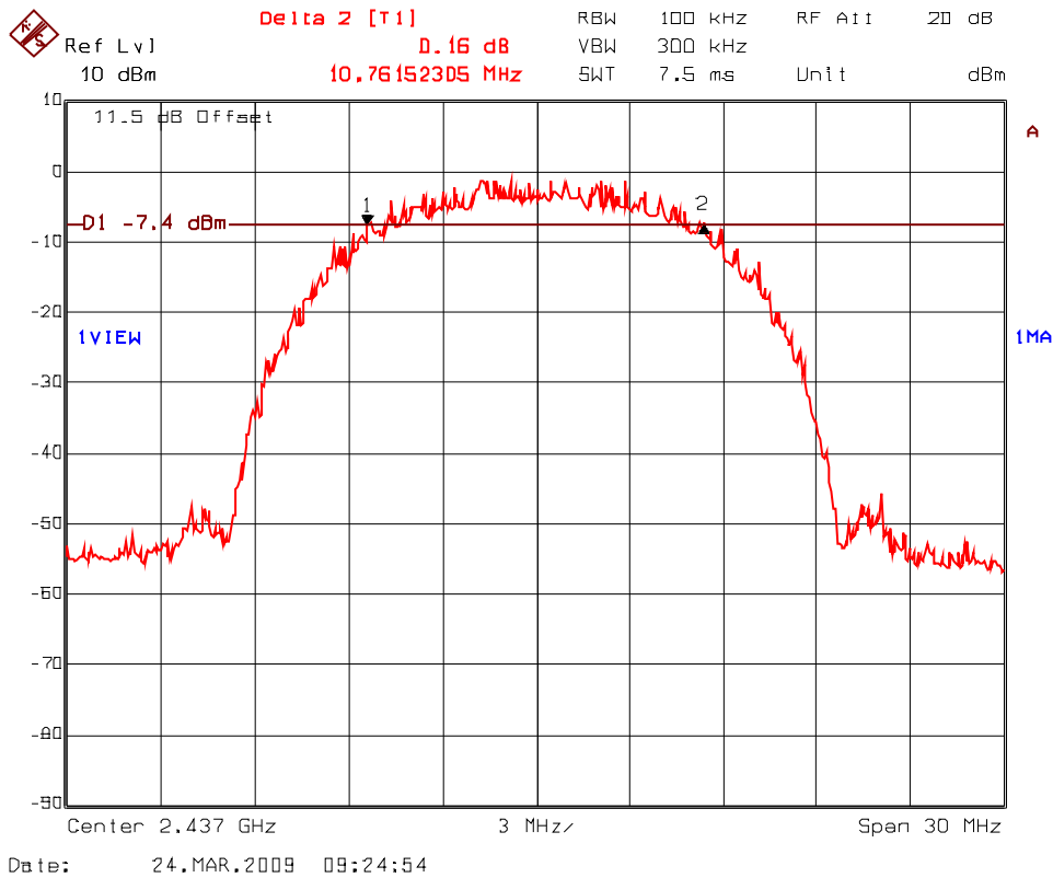
Plot 5.5.4.8. 6 dB Bandwidth Frequency: 2437 MHz; Modulation: CCK at 11 Mbps
