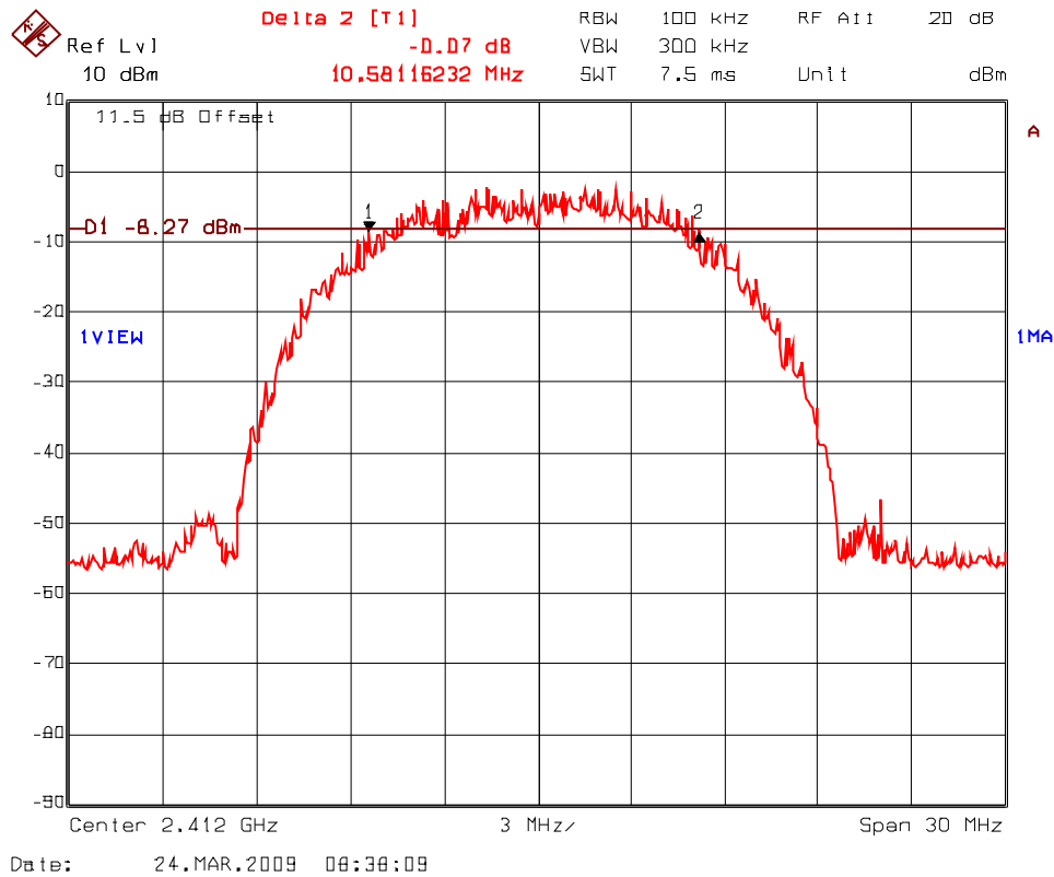
Plot 5.5.4.1. 6 dB Bandwidth Frequency: 2412 MHz; Modulation: DBPSK at 1 Mbps
