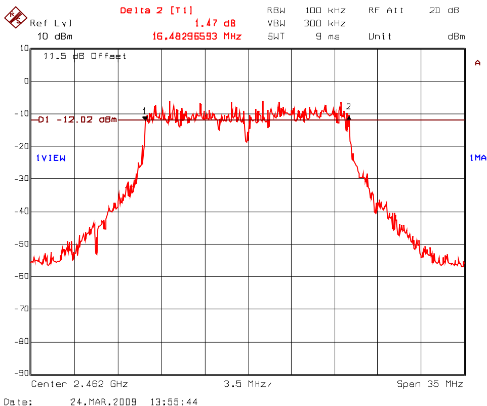
Plot 5.5.4.21. 6 dB Bandwidth Frequency: 2462 MHz; Modulation: 64QAM at 54 Mbps
