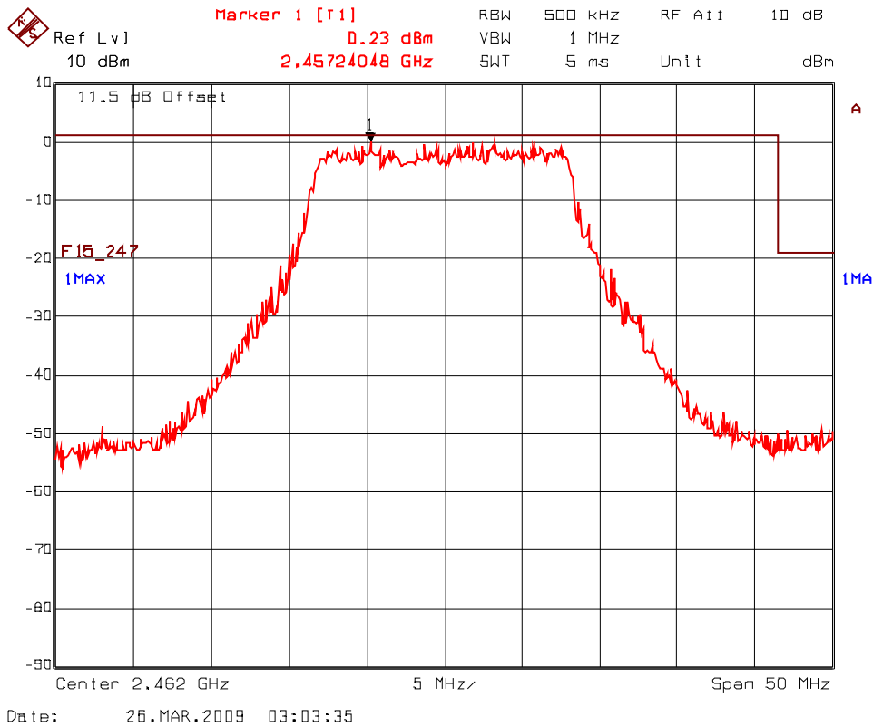
Plot 5.7.4.1.4. Band-Edge RF Conducted Emissions, 802.11g Mode High End of Frequency Band 2412 -2462 MHz
