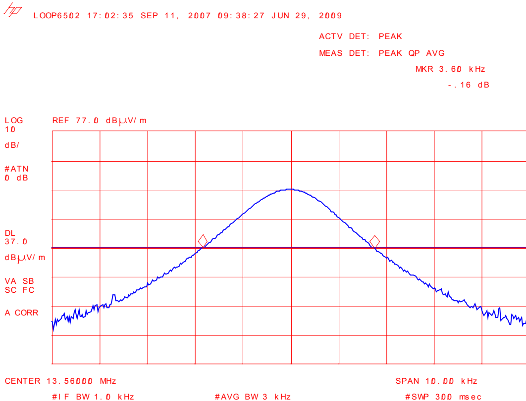
Plot 5.5.3.1. 20 dB Bandwidth Test Frequency: 13.56 MHz
