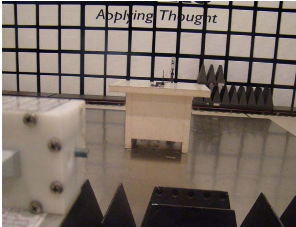
Test setup-Radiated Emissions 18GHz – 26.5GHz
