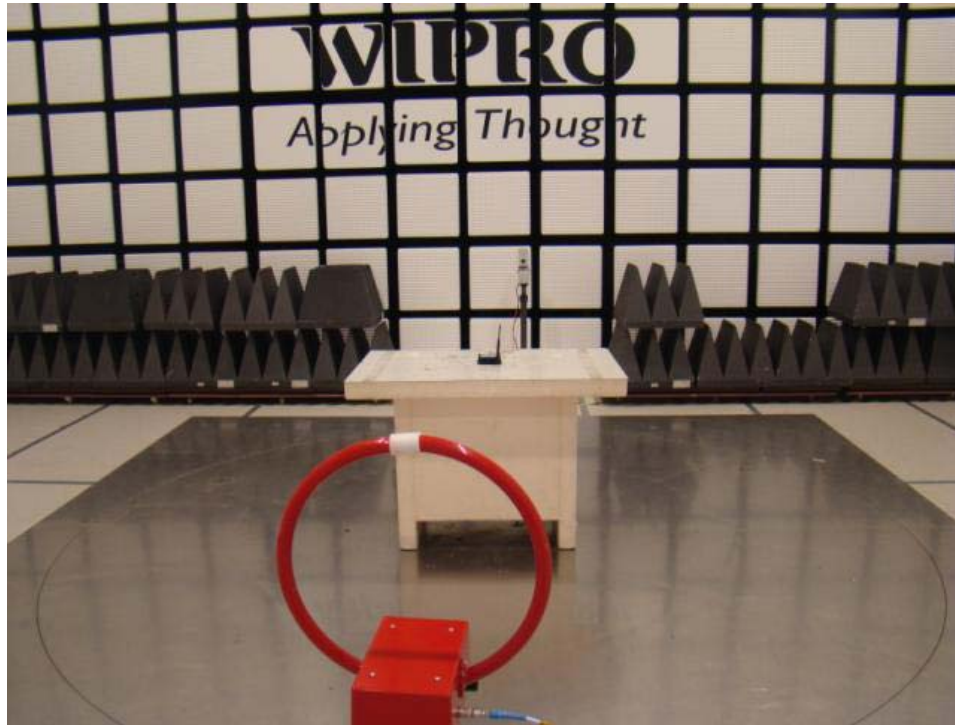
Test setup-Radiated Emissions 9KHz-30MHz
