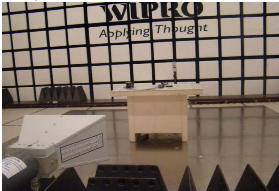
Test setup-Radiated Emissions 1GHz – 18GHz
