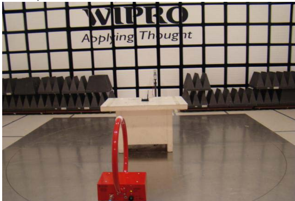
Test setup-Radiated Emissions 9KHz – 30MHz
