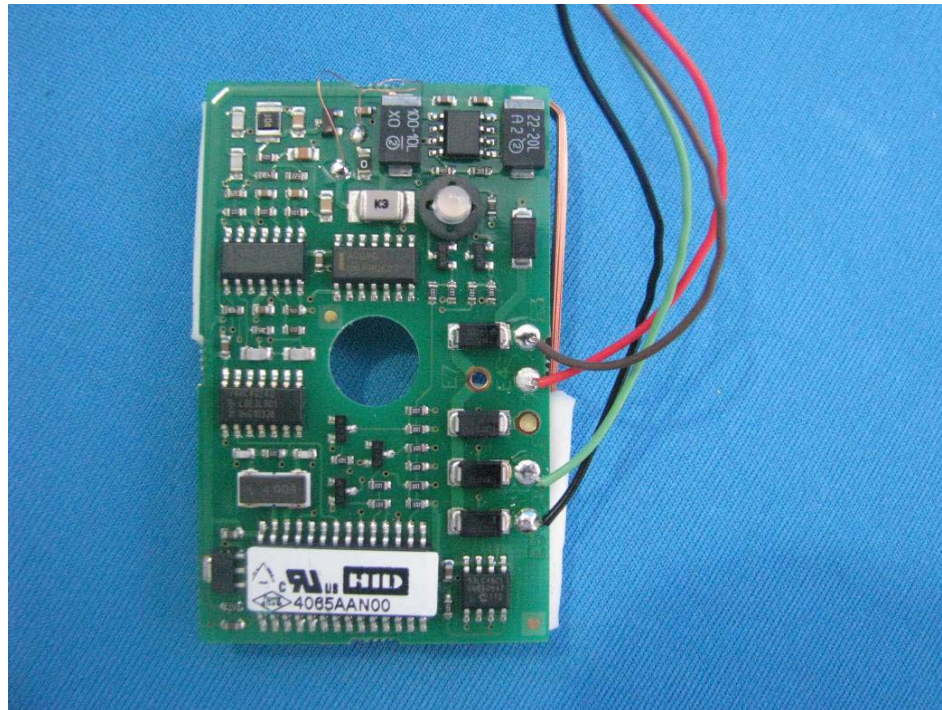
Reader PCB
