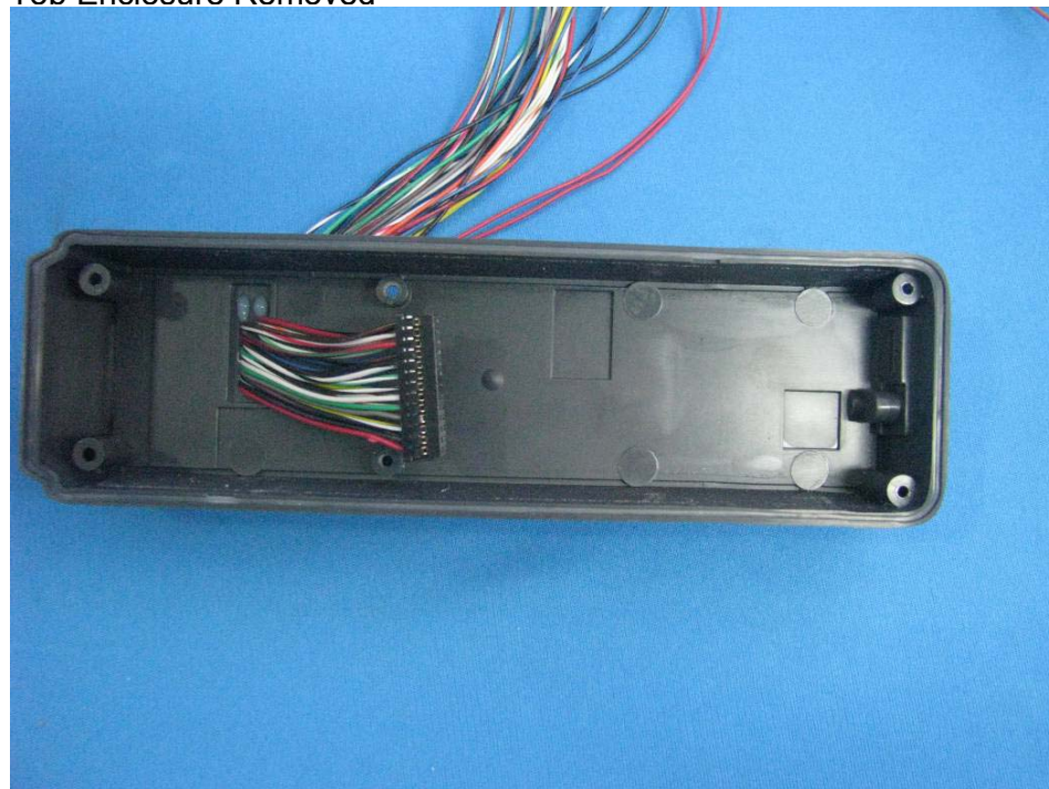
Bottom View of top Enclosure
