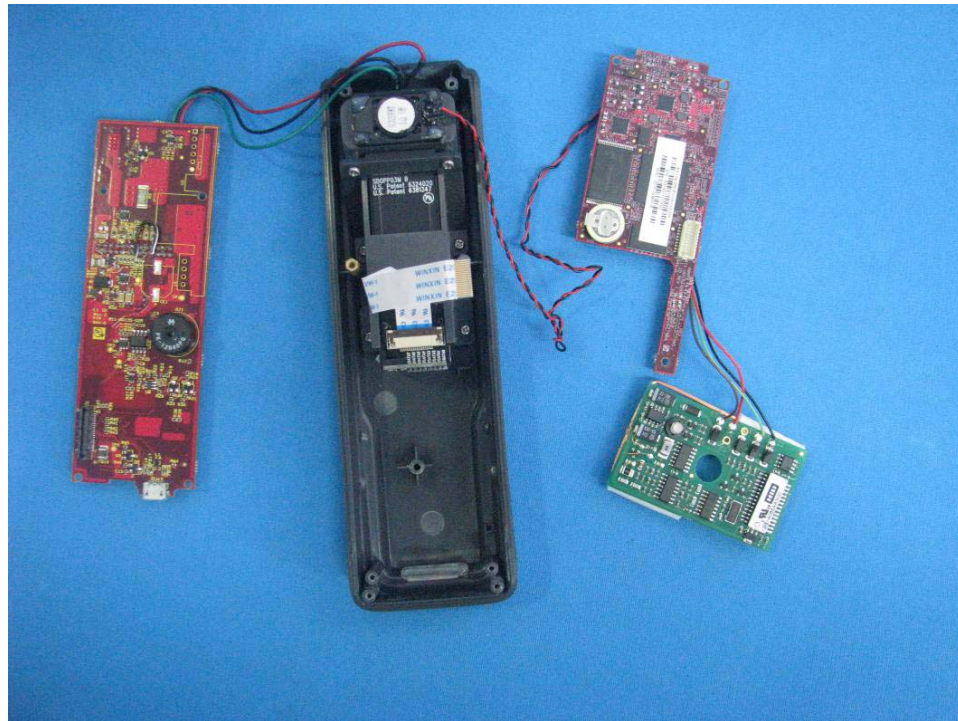
All PCBs removed
