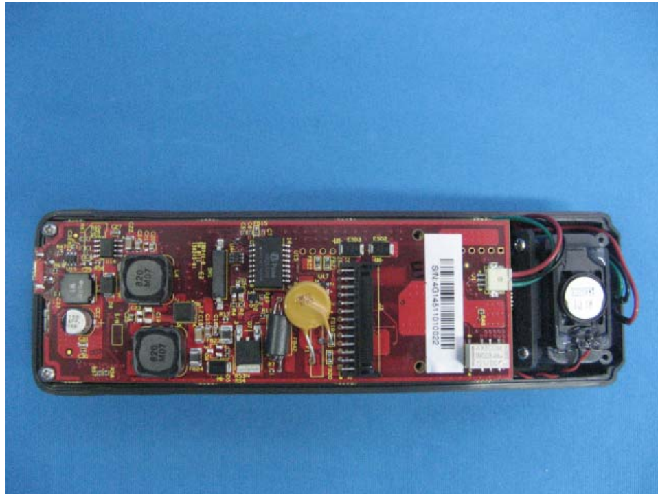
Top Enclosure Removed
