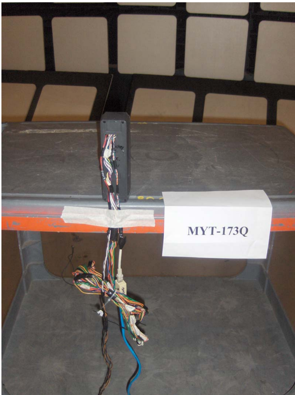
Radiated Emissions at 10 m or 3 m Distance (rear view)
