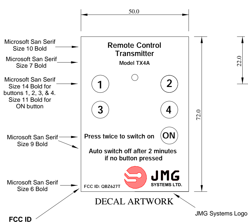
DECAL DIMENSIONS
