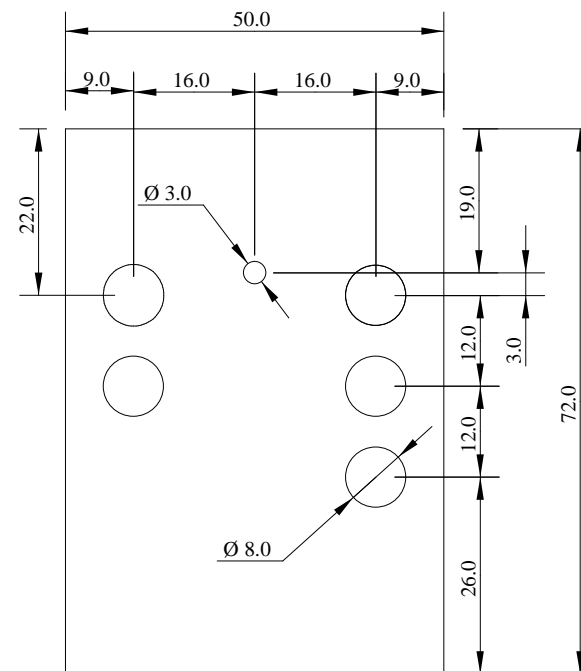
DECAL DIMENSIONS
