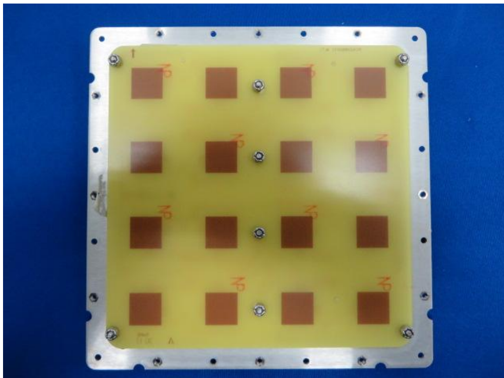
(18) EUT Photo (Antenna MT-485053/SVH/A)
