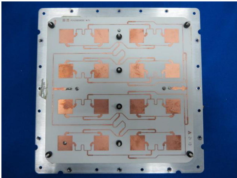
(20) EUT Photo (Antenna MT-485053/SVH/A)
