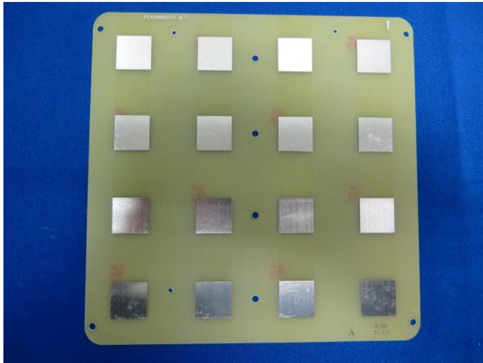
(29) EUT Photo (Antenna MT-485053/SVH/A)
