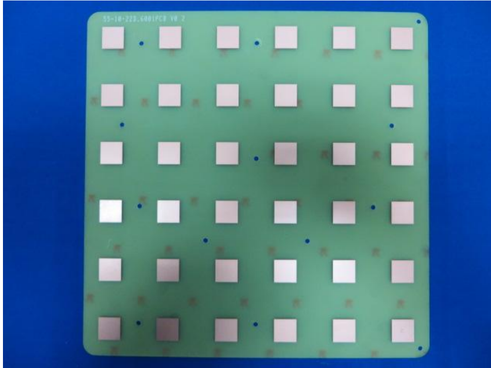
(22) EUT Photo (Antenna MT-485053/SVH/A)
