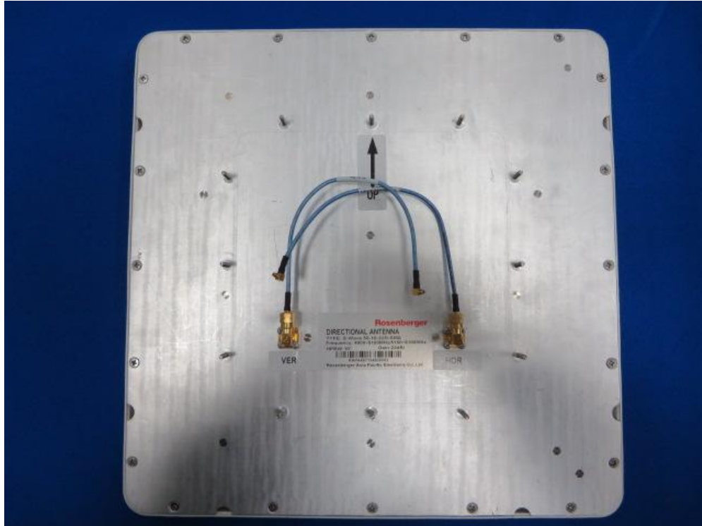
(16) EUT Photo (Antenna S-Wave 55-10-22D-SMA)
