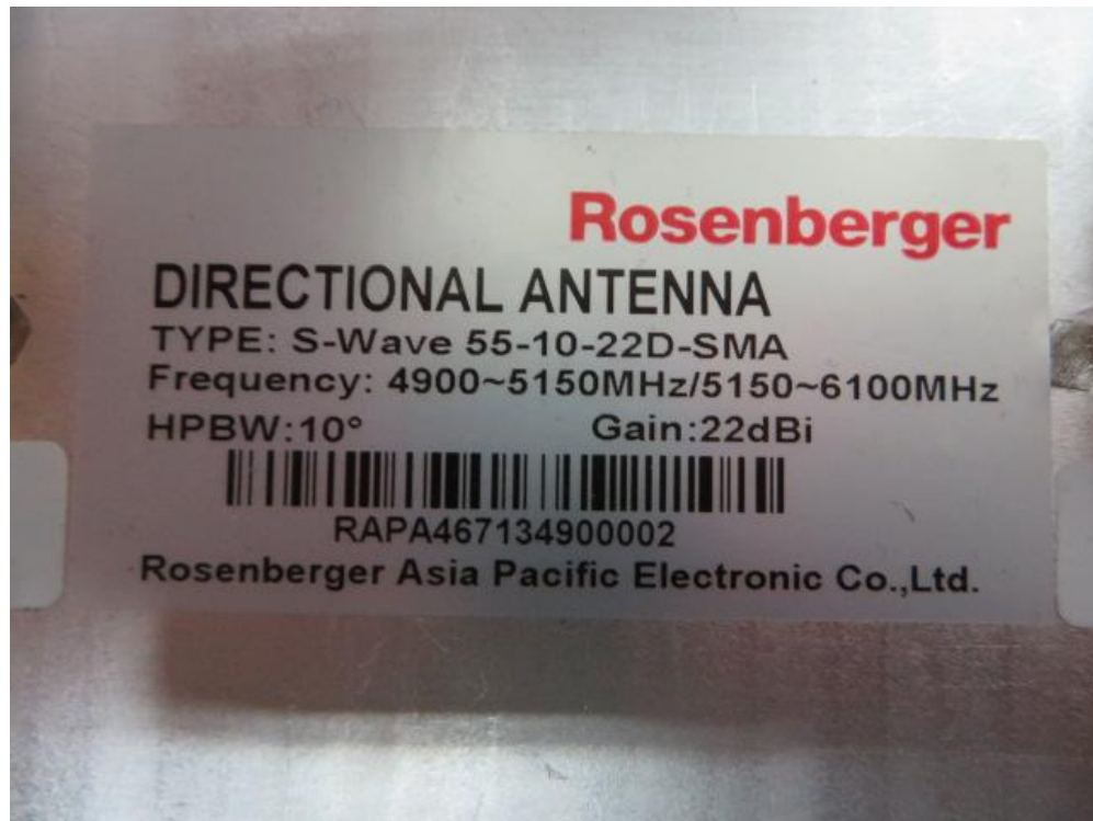
(17) EUT Photo (Antenna S-Wave 55-10-22D-SMA)
