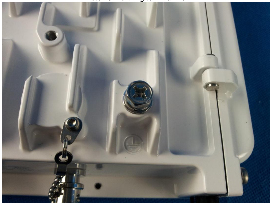
Photo 10. Earthing terminal View
