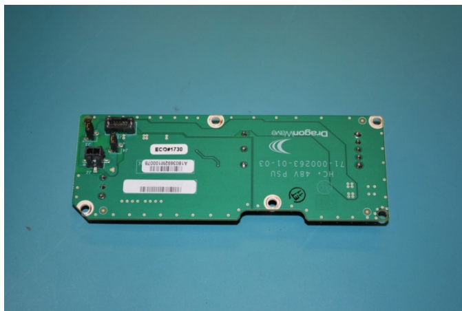
PSU Card bottom
