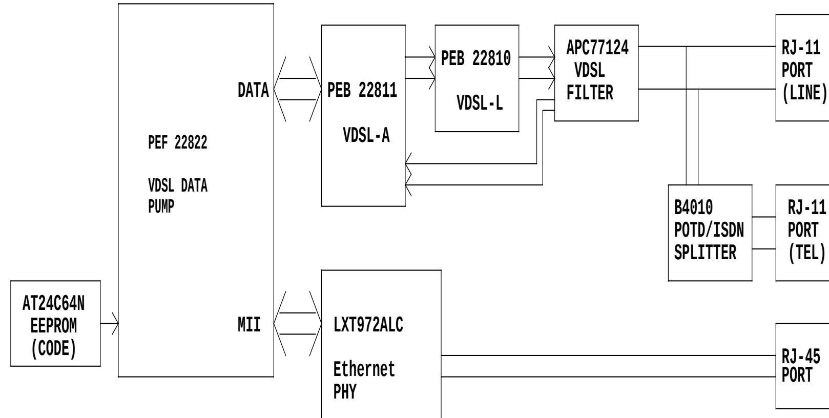
1. Block Diagram
