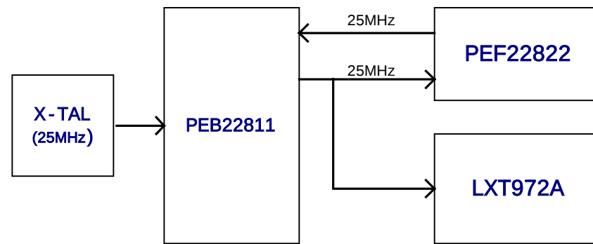
2. CLOCK Stucture
