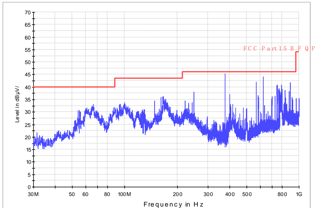
Field strength 30M-1GHz 1F 3m chamber
