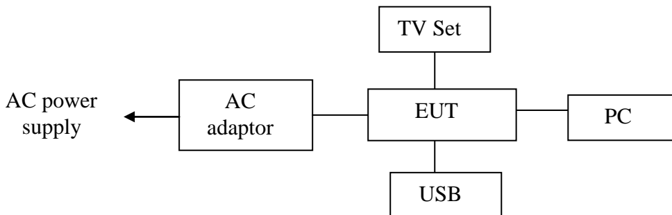
Figure 1 EUT setup
