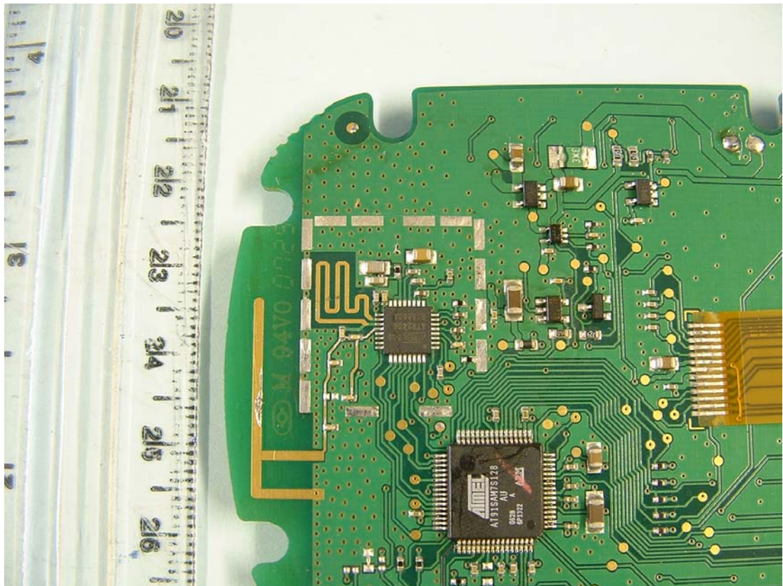
RF SECTION CAN REMOVED
