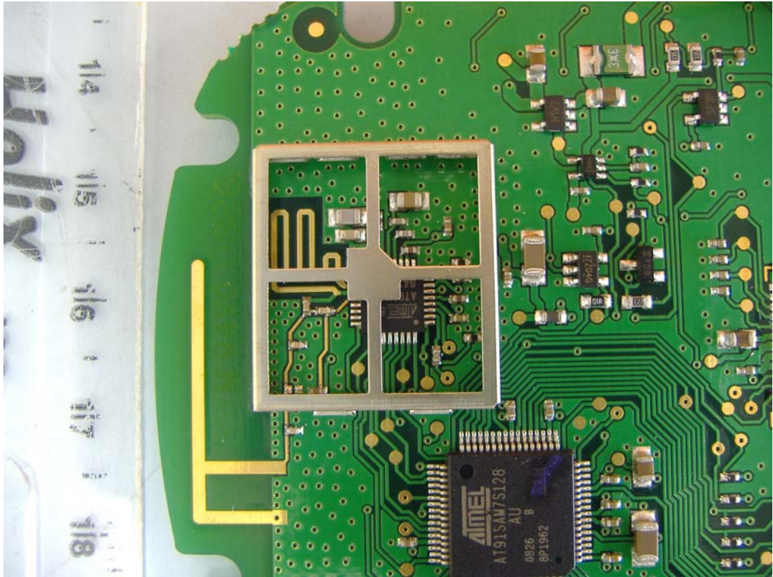
RF SECTION CAN LID REMOVED
