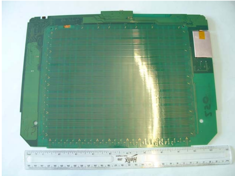
Track Side Of PCB
