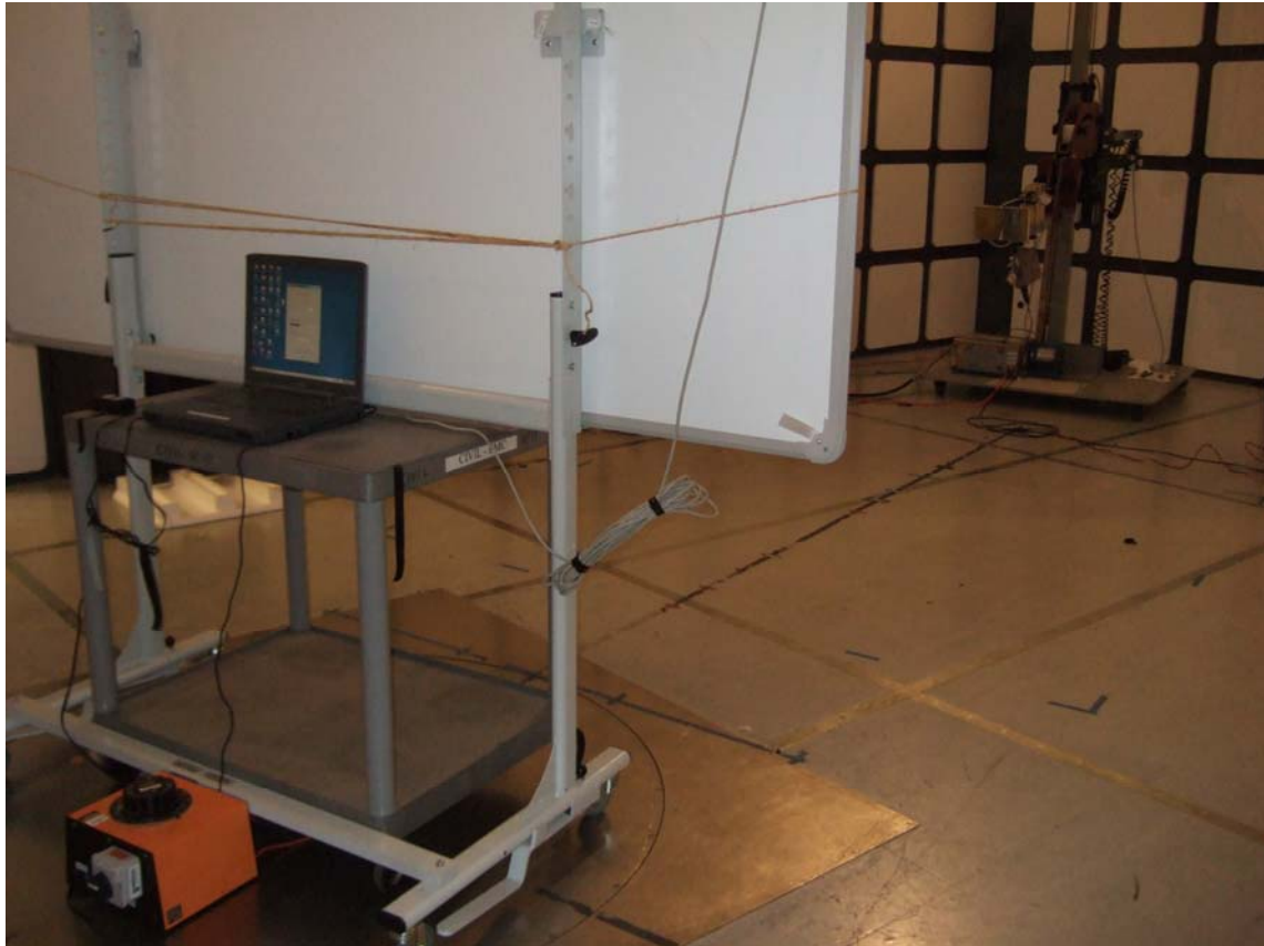
Radiated Emissions
