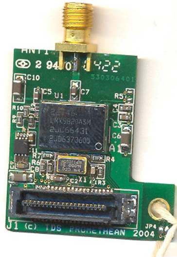
Component view (modified for test With antenna connector)
