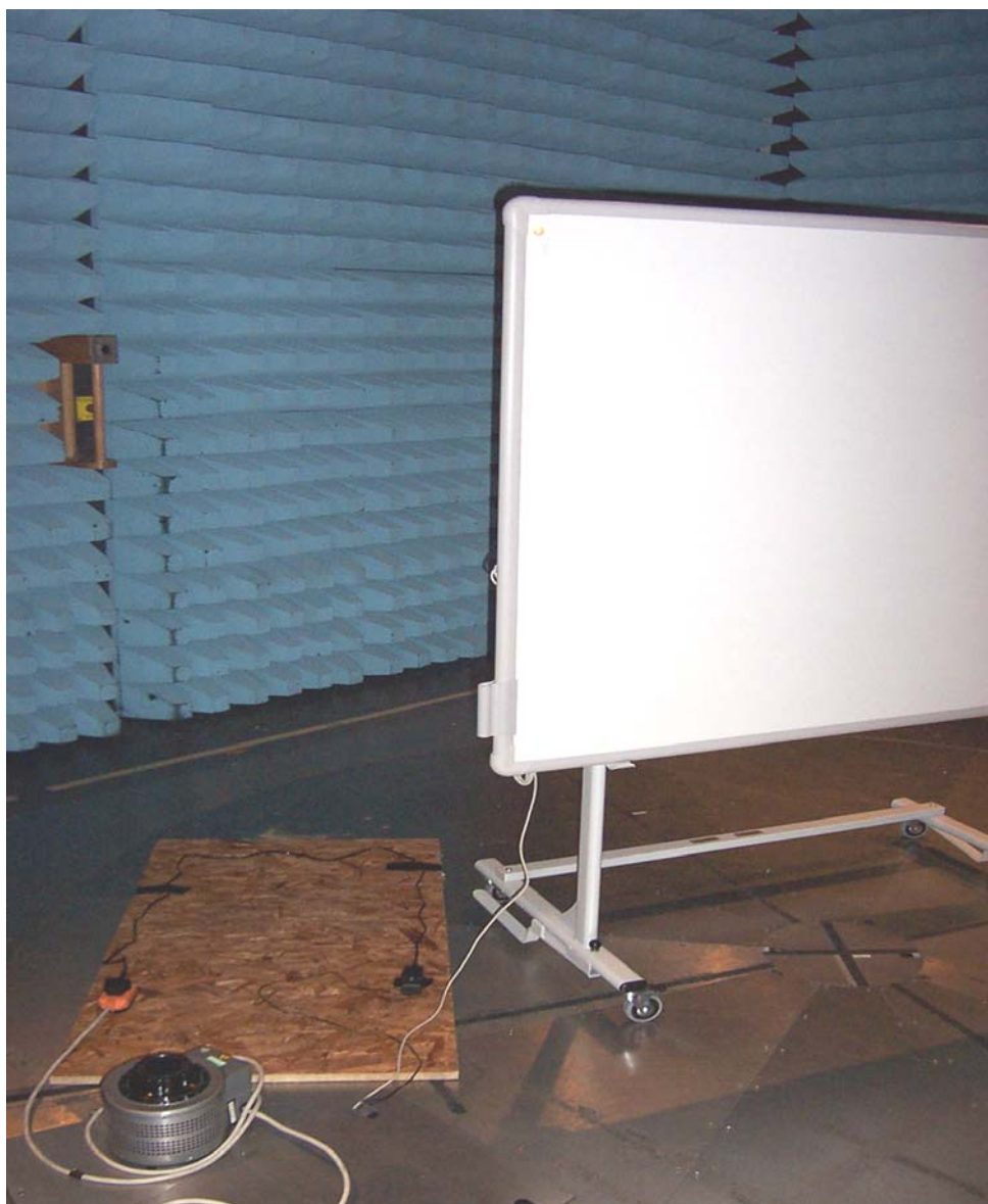
Radiated Emissions Set Up Photograph
