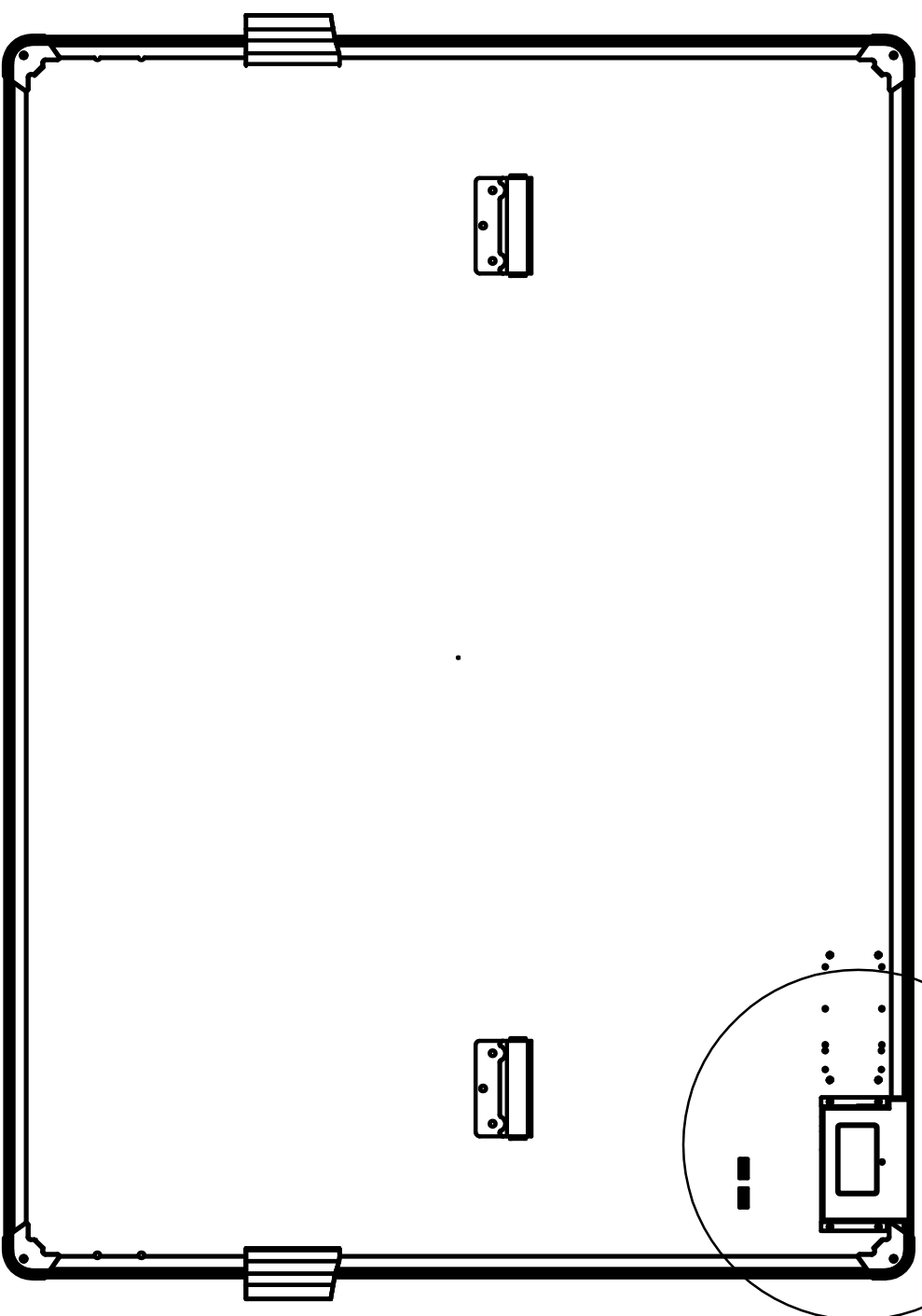
REAR VIEW OF WHITEBOARD SHOWING ELECTRONICS POD AND LABEL POSITION SCALE 1:2
