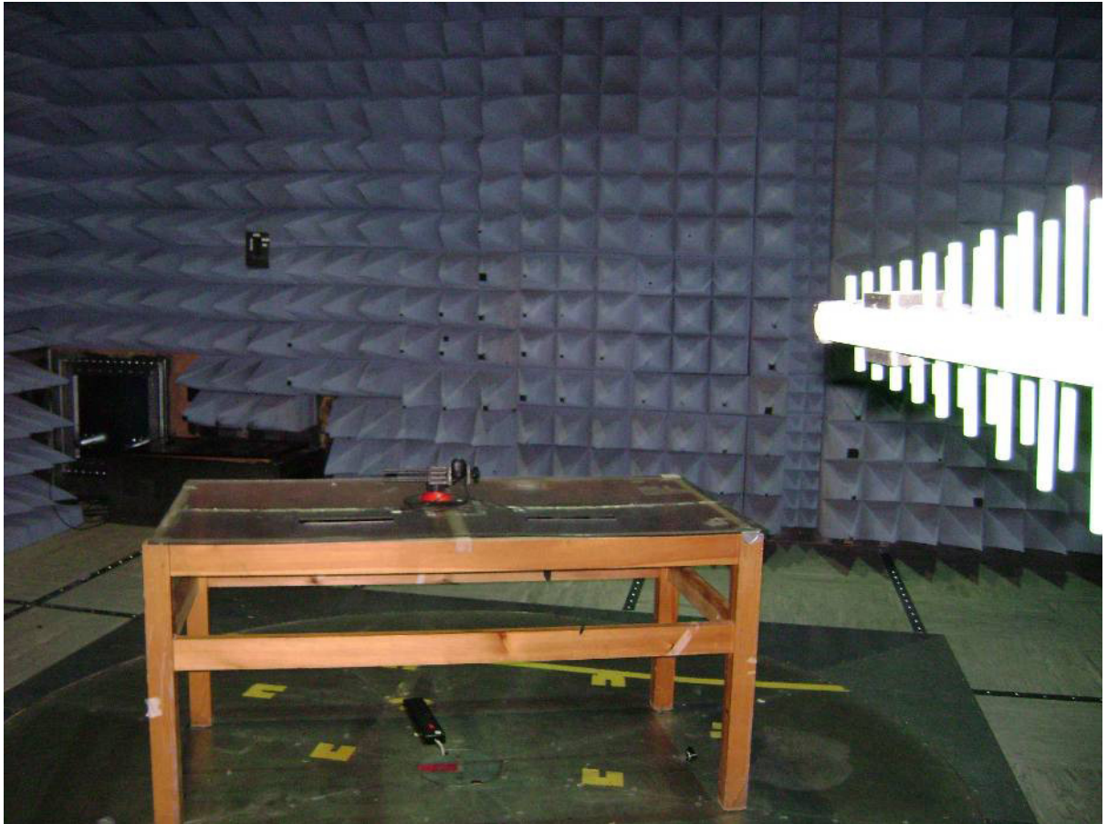
Receiver radiated emissions below 1GHz
