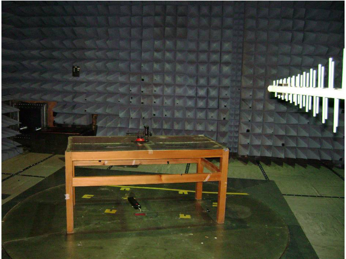
Transmitter radiated emissions below 1GHz
