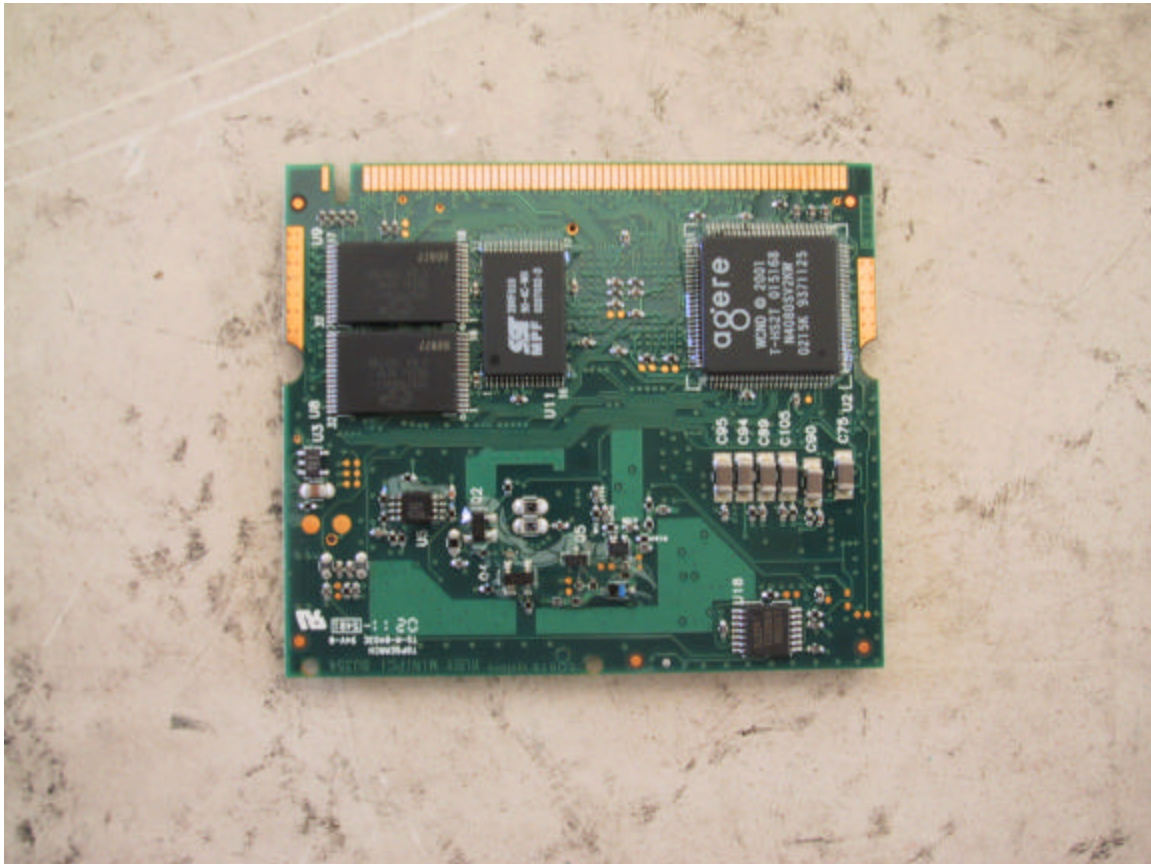
Radio PCB – Bottom Side
