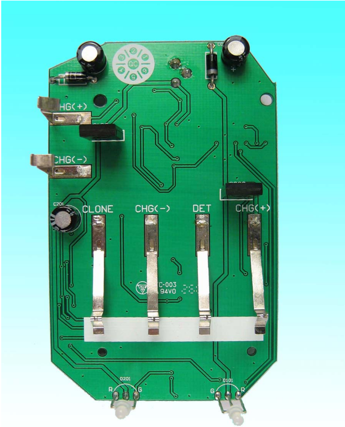
CHARGER – BOTTOM VIEW
