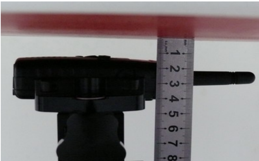
Picture 4: Body, The EUT display towards phantom, the distance from EUT to the bottom of the Phantom is 15mm
