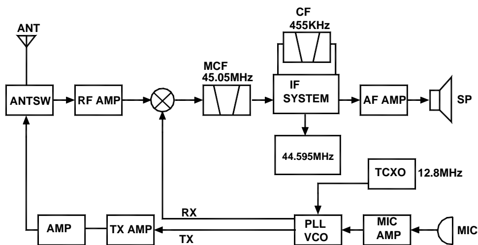
Figure 1 frequency configuration
