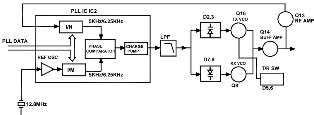
Figure 4 PLL circuit
